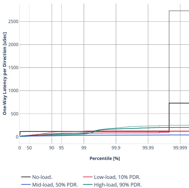
Latency: rdma-ethip6-ip6scale200k
