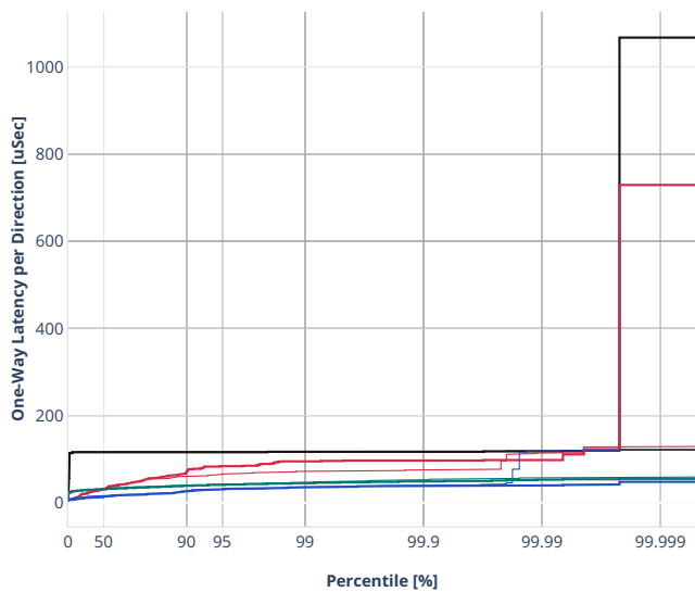
Latency: rdma-dot1q-l2bdbasemacrln
