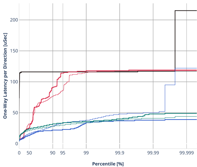
Latency: rdma-ethip4-ip4scale2m-rnd
