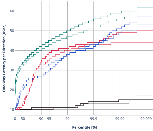
Latency: eth-l2bdscale100kmac1rn
