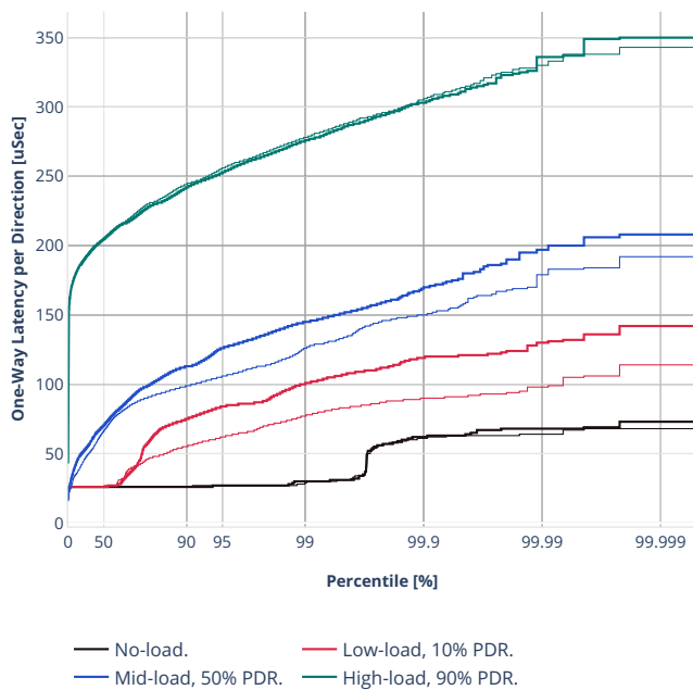
Latency: eth-l2xcbase-eth-2vhostvr1024-1vm
