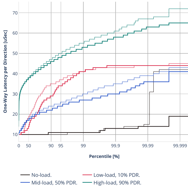
Latency: eth-l2bdscale10kmaclrn
