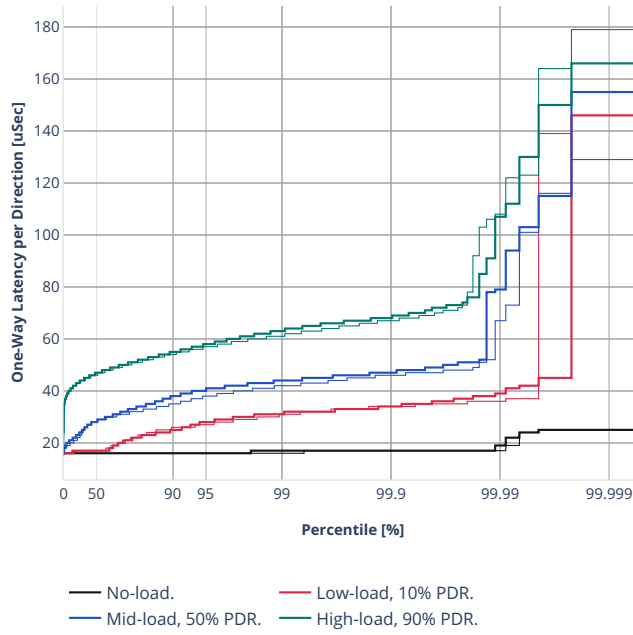
Latency: avf-ethip4-ip4scale2m
