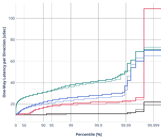
Latency: avf-ethip4-ip4scale200k-rnd
