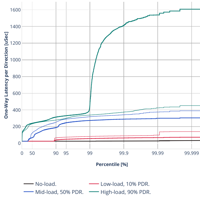
Latency: avf-ethip4ipsec10000tnlsw-ip4base-int-aes256gcm
