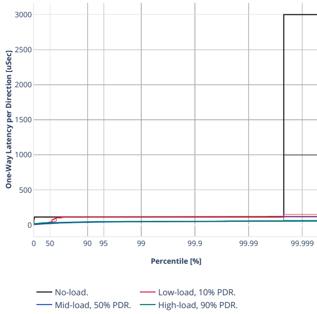
Latency: rdma-ethip4udp-nat44det-h1-p1-s1
