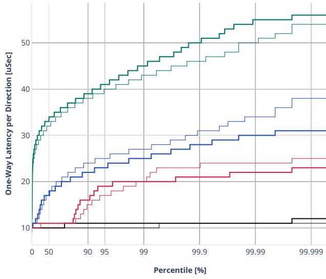
Latency: avf-eth-l2bdscale100kmac1rn
