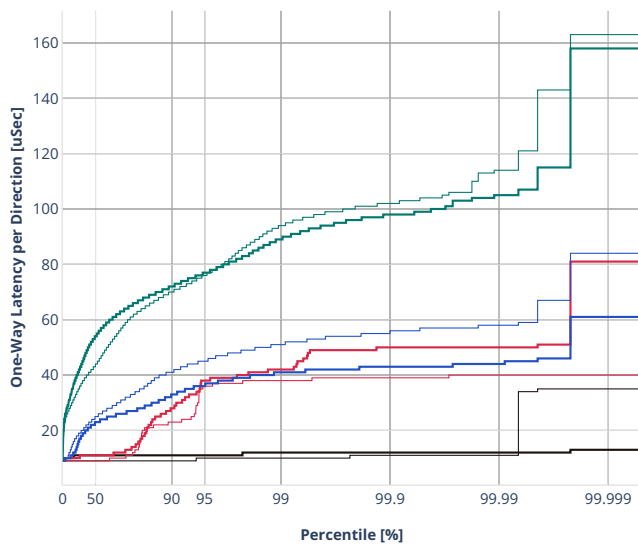
Latency: ethip4udp-ip4base-iac150sl-10kflows
