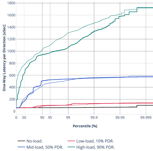
Latency: ethip4ipsec10000tnlsw-ip4base-int-aes128cbc-hmac512sha
