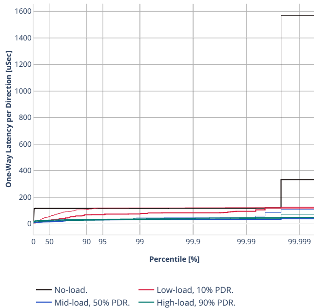
Latency: rdma-eth-l2bdscale10kmaclrn
