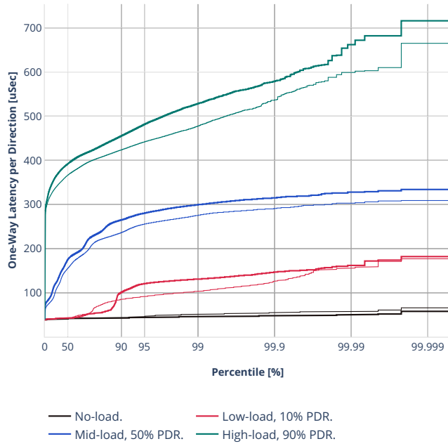
Latency: ethip4-ip4base-eth-2vhostvr1024-1vm-vppip4
