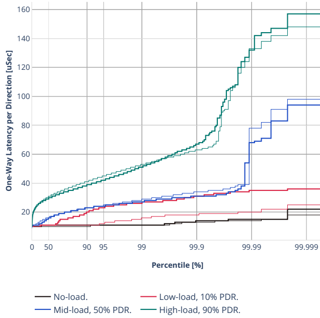
Latency: avf-ethip6-ip6scale2m
