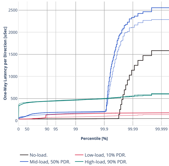
Latency: ethip6srhip6-ip6base-srv6proxy-masq
