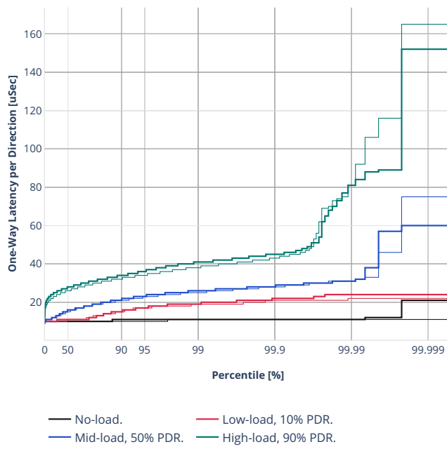
Latency: avf-ethip4-ip4scale2m
