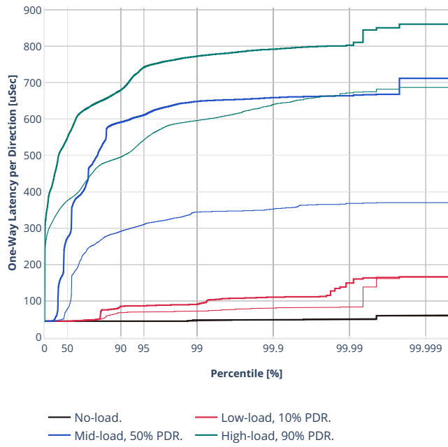
Latency: avf-ethip4ipsec1000tnlsw-ip4base-int-aes128cbc-hmac512sha
