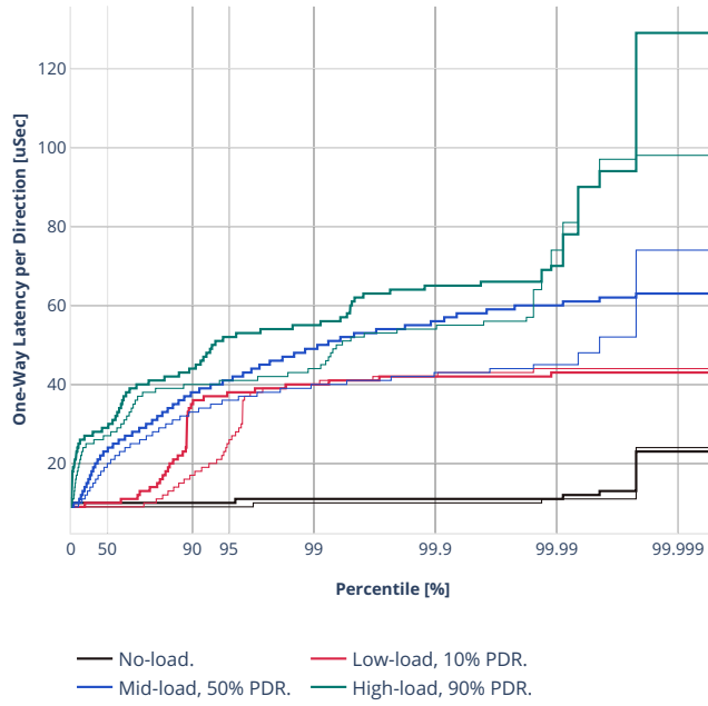
Latency: ethip6-ip6base
