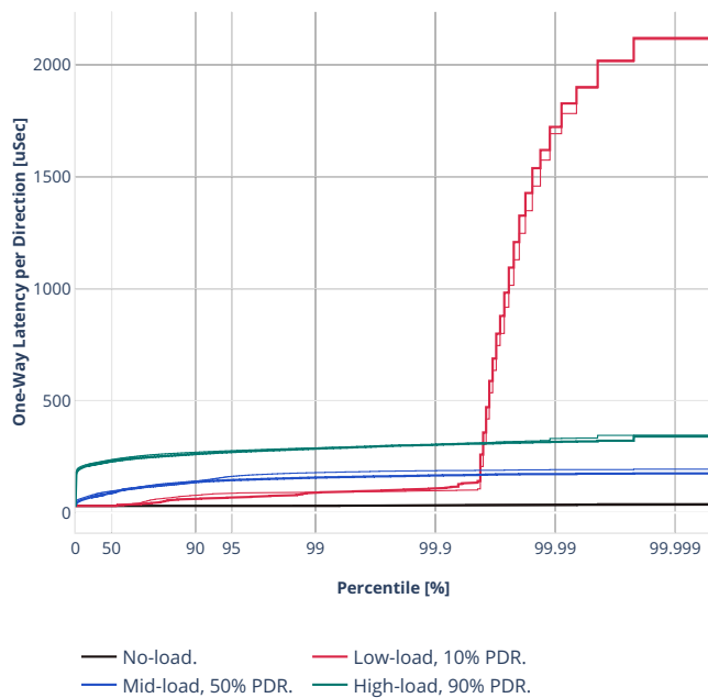
Latency: ethip4vxlan-l2bdbasemaclrn
