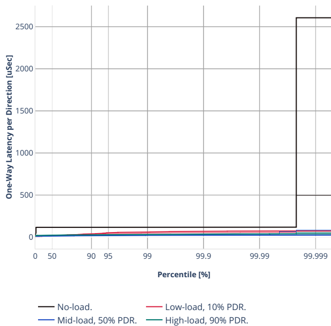
Latency: rdma-eth-l2xcbase
