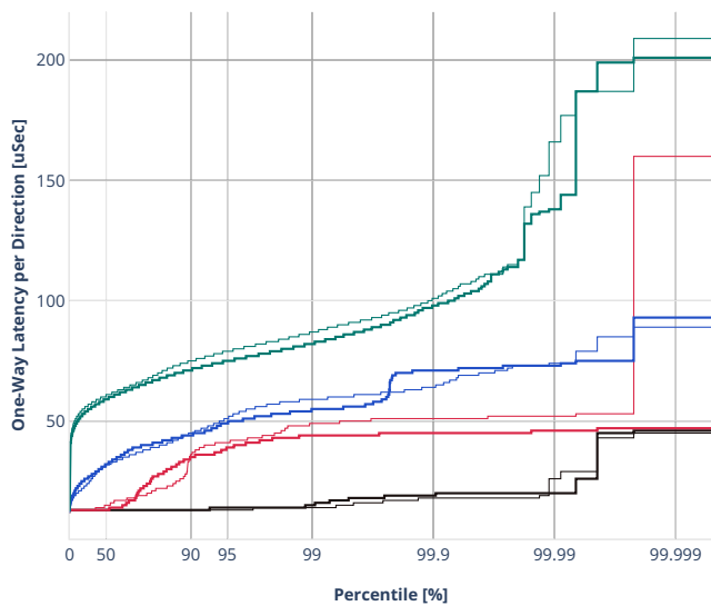
Latency: eth-l2xcbase-eth-2vhostvr1024-1vm-vppl2xc
