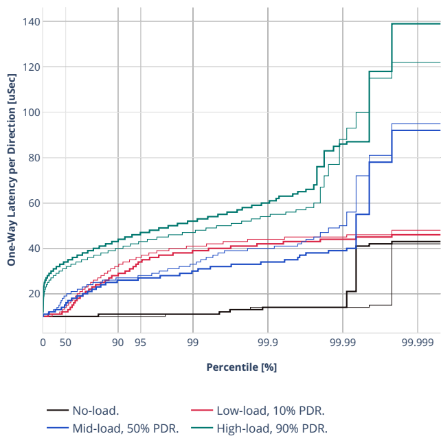
Latency: eth-l2bdscale100kmacirn
