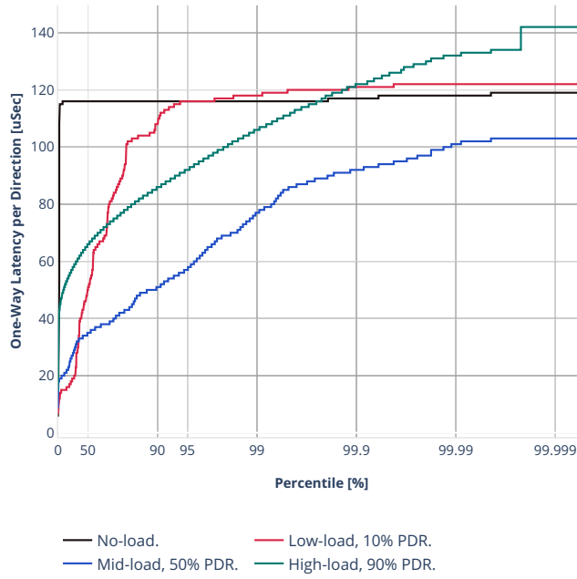
Latency: rdma-dot1q-l2xcbase-eth-2vhostvr1024-1vm
