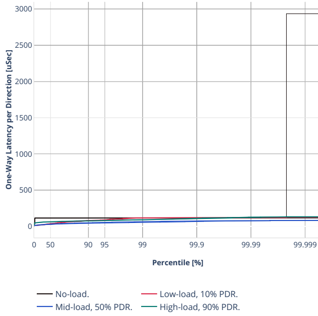
Latency: rdma-eth-l2xcbase-eth-2vhostvr1024-1vm-vppl2xc
