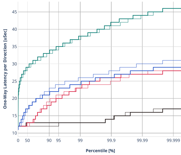
Latency: avf-ethip4-ip4scale20k
