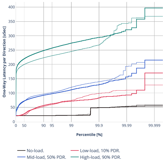
Latency: ethip4-ip4base-eth-2vhostvr1024-1vm
