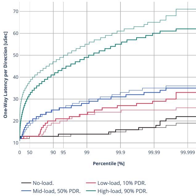
Latency: avf-ethip6-ip6scale200k
