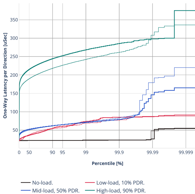
Latency: eth-l2xcbase-eth-2memif-1lxc
