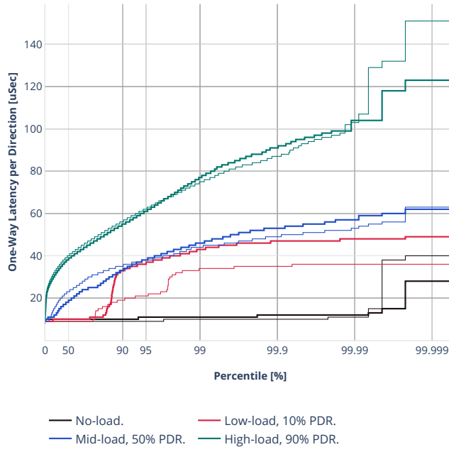
Latency: eth-l2bdscale1mmaclrn
