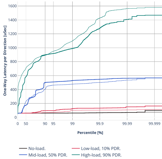
Latency: ethip4ipsec1000tnlsw-ip4base-int-aes128cbc-hmac512sha
