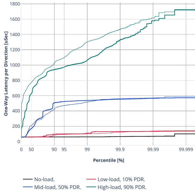
Latency: ethip4ipsec10000tnlsw-ip4base-int-aes128cbc-hmac512sha
