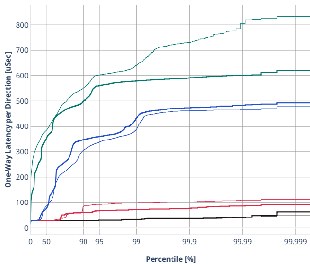
Latency: ethip4ipsec4tnlsw-ip4base-int-aes256gcm
