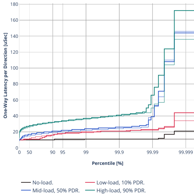
Latency: avf-ethip4-ip4base
