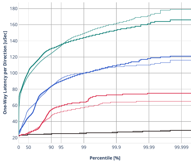
Latency: ethip4udp-ip4base-oacl50sf-10kflows
