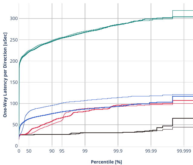
Latency: ethip6srhip6-ip6base-srv6proxy-masq
