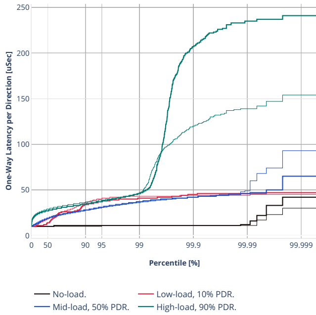
Latency: ethip6-ip6scale200k-rnd
