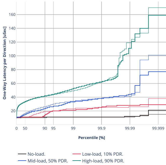
Latency: avf-ethip6-ip6scale2m-rnd
