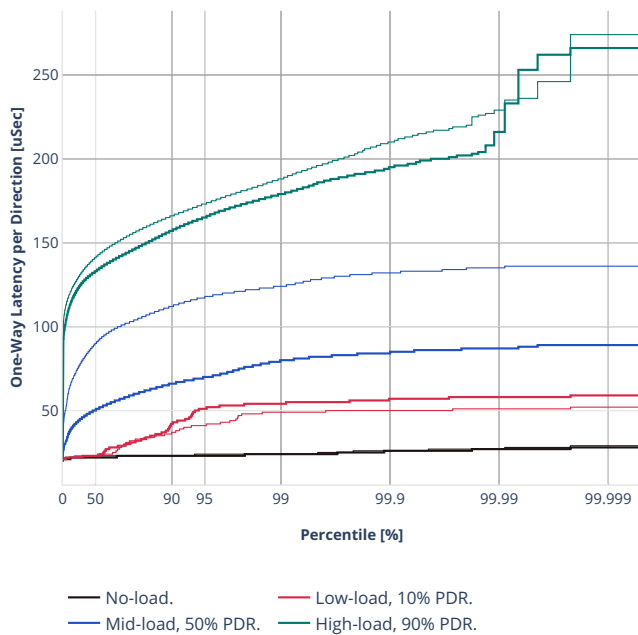
Latency: ethip4-ip4scale200k
