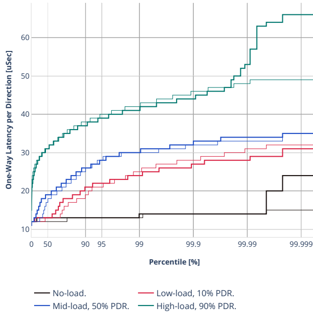
Latency: avf-ethip6-ip6scale20k-rnd
