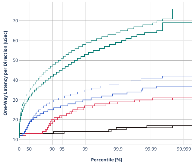
Latency: avf-ethip6-ip6scale2m
