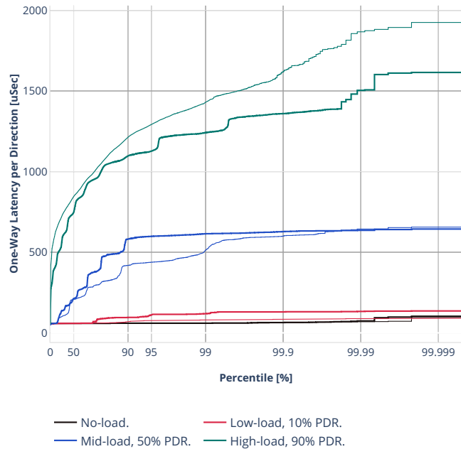
Latency: ethip4ipsec1000tnlhw-ip4base-int-aes128cbc-hmac512sha
