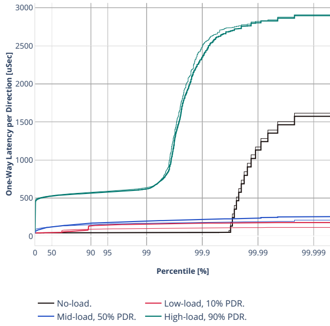
Latency: ethip4-ip4base-eth-2memif-1dcr
