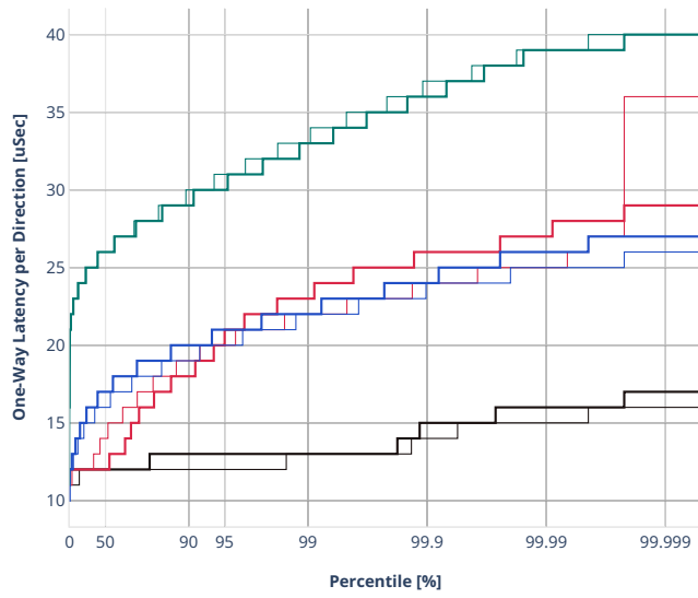
Latency: avf-eth-l2xcbase
