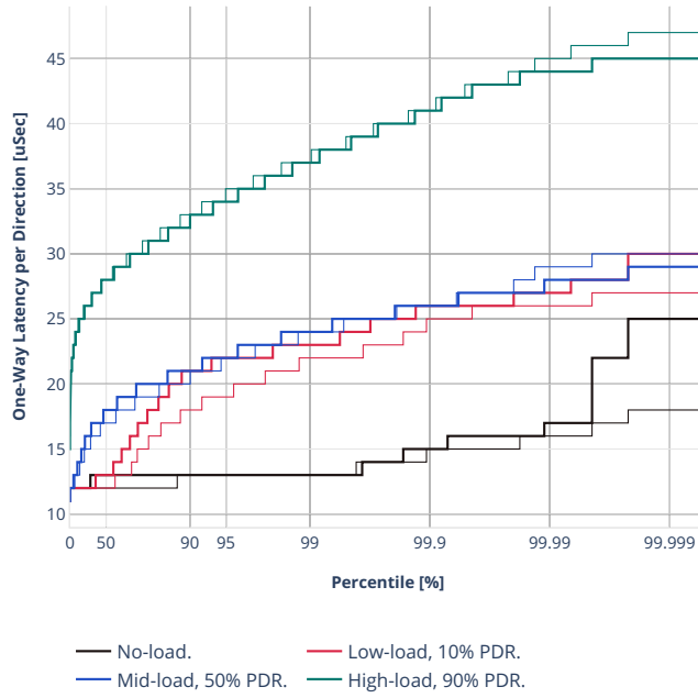
Latency: avf-eth-l2bdbasemaclrn
