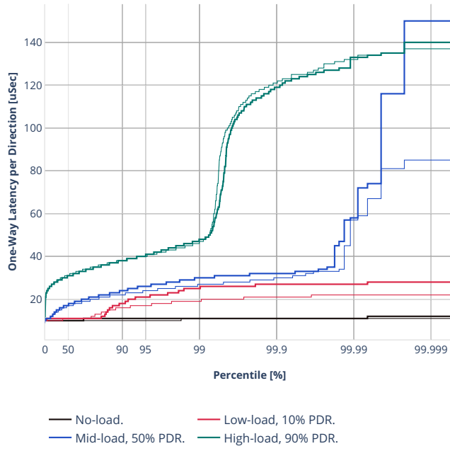
Latency: avf-ethip6-ip6scale200k-rnd
