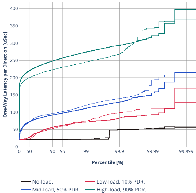
Latency: ethip4-ip4base-eth-2vhostvr1024-1vm
