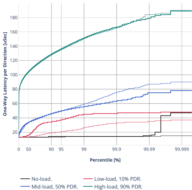
Latency: eth-l2xcbase-eth-2memif-1dcr
