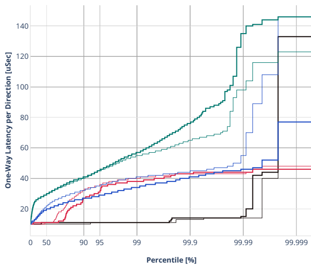
Latency: ethip6-ip6scale2m
