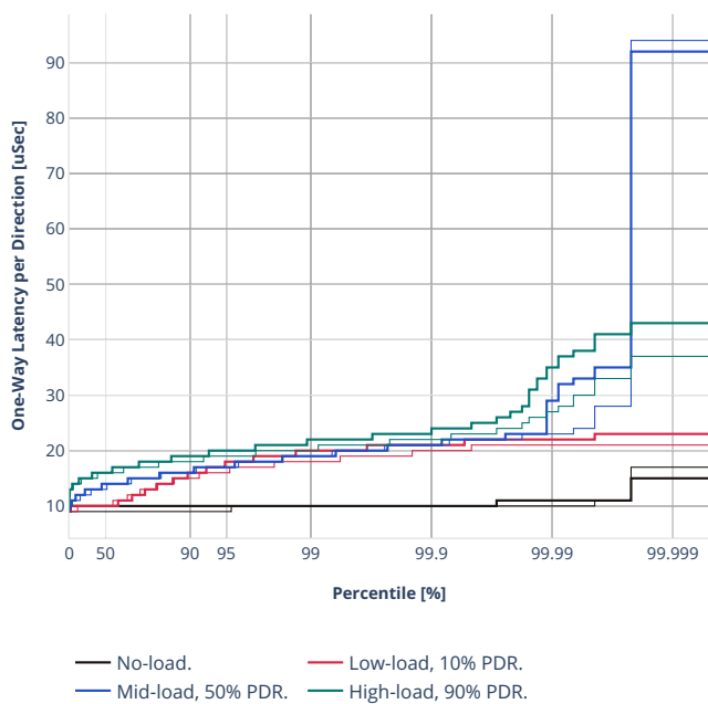
Latency: avf-eth-l2patch
