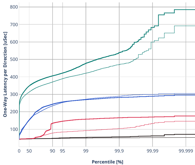
Latency: eth-l2bdbasemaclrn-eth-2vhostvr1024-1vm-vppl2xc
