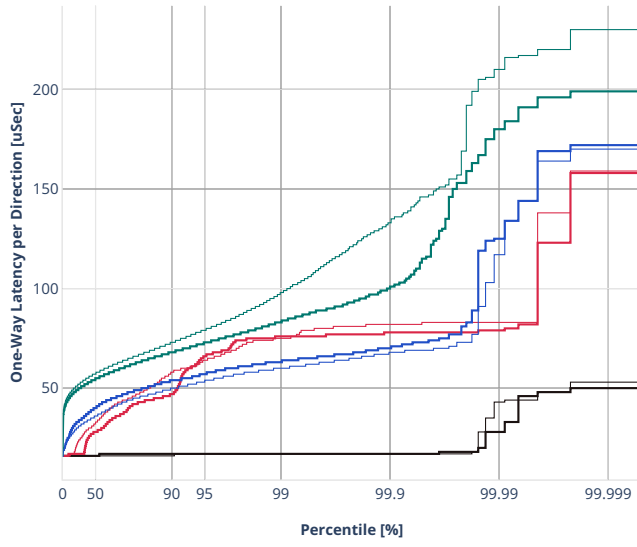
Latency: ethip6-ip6scale2m
