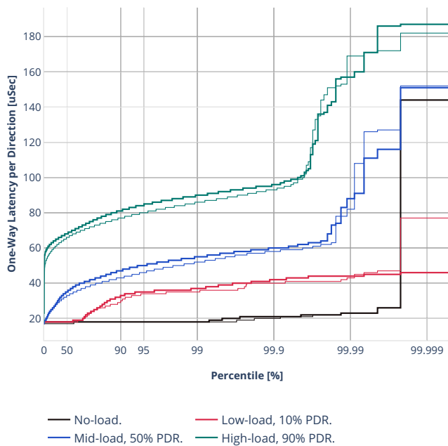
Latency: avf-ethip4vlan-l2bdbasemacrn
