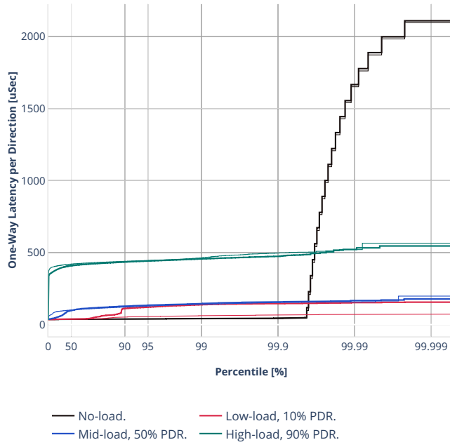
Latency: ethip6srhip6-ip6base-srv6proxy-dyn
