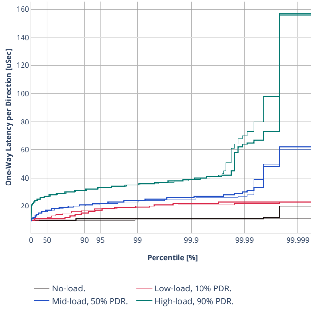
Latency: avf-eth-l2bdbasemaclrn
