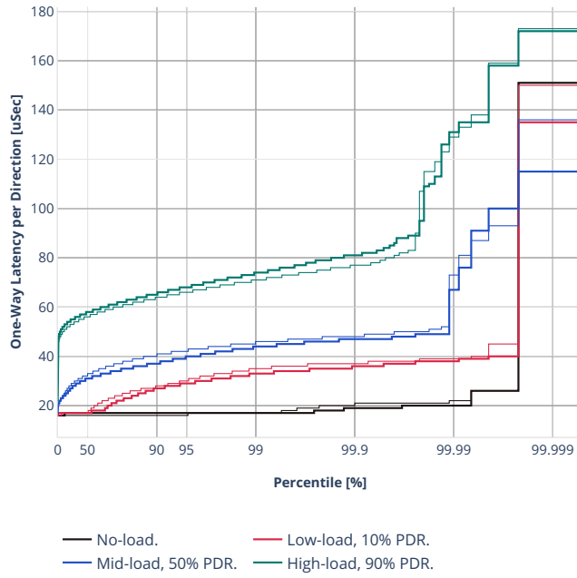
Latency: avf-dot1q-l2bdbasemaclrn
