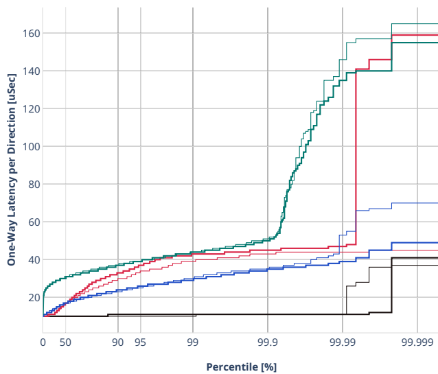
Latency: ethip4-ip4scale20k-rnd
