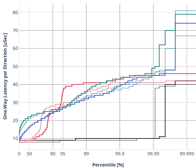
Latency: eth-l2patch
