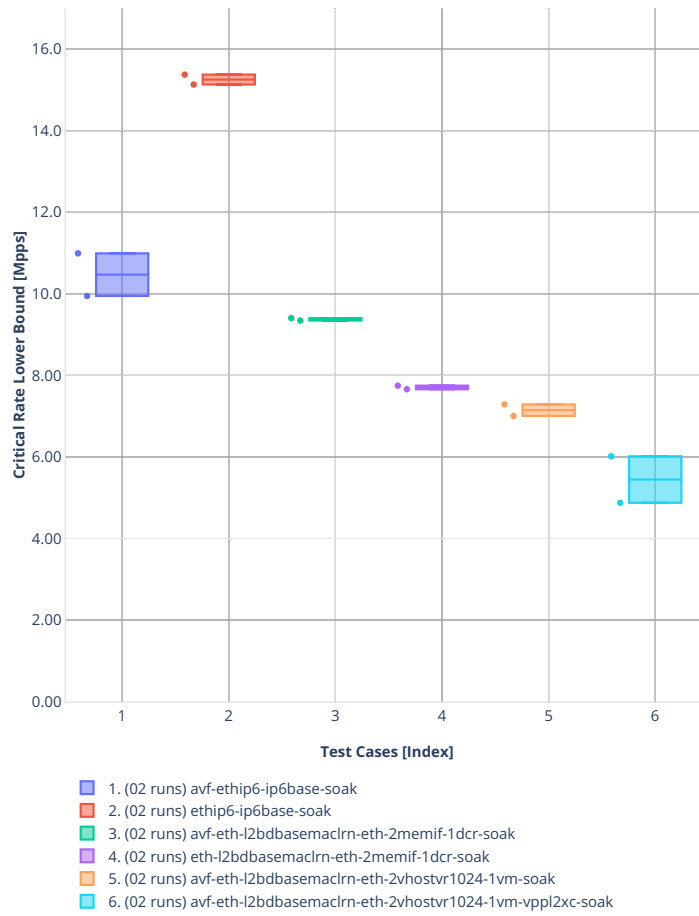
Throughput: 30 Minutes Soak Test (PLRsearch)
