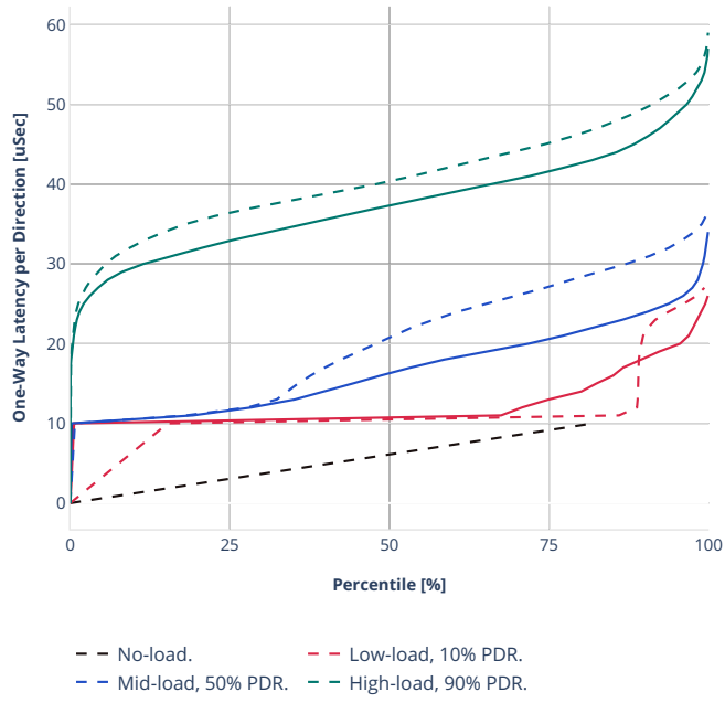
Latency: avf-ethip4udp-nat44det-h1-p1-s1
