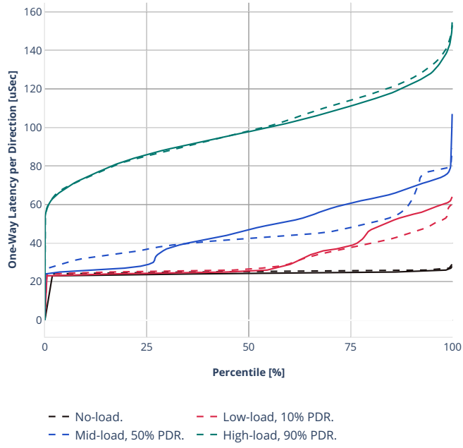
Latency: eth-l2bdbasemaclrn-iacl50sl-10kflows
