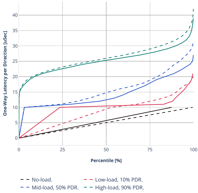
Latency: avf-ethip4-ip4scale200k-rnd
