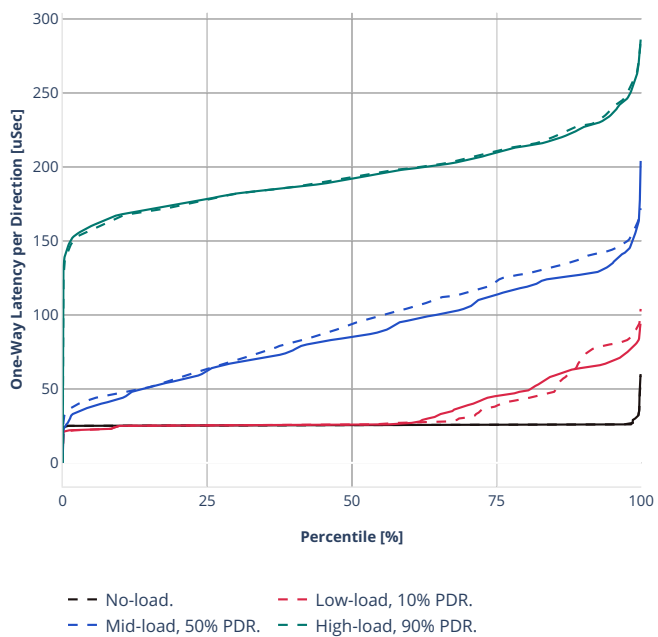
Latency: eth-l2xcbase-eth-2vhostvr1024-1vm
