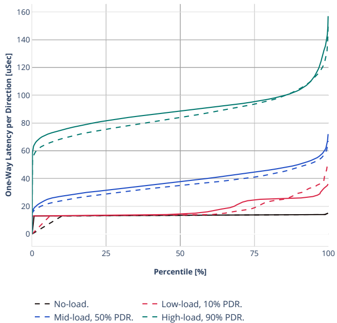
Latency: eth-l2bdbasemaclrn-eth-2memif-1dcr
