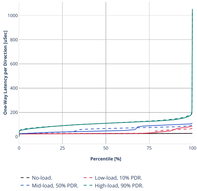
Latency: eth-l2bdbasemaclrn-oac150sf-10kflows
