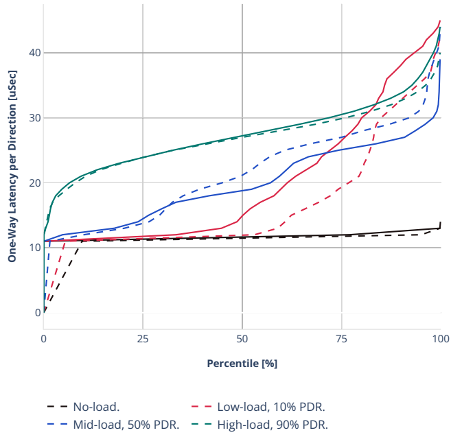
Latency: ethip4-ip4scale2m
