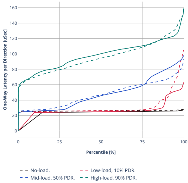
Latency: eth-l2bdbasemaclrn-oacl50sl-10kflows
