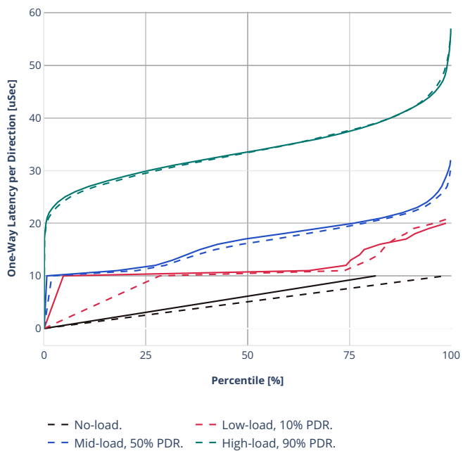
Latency: avf-eth-l2bdscale100kmac1rn
