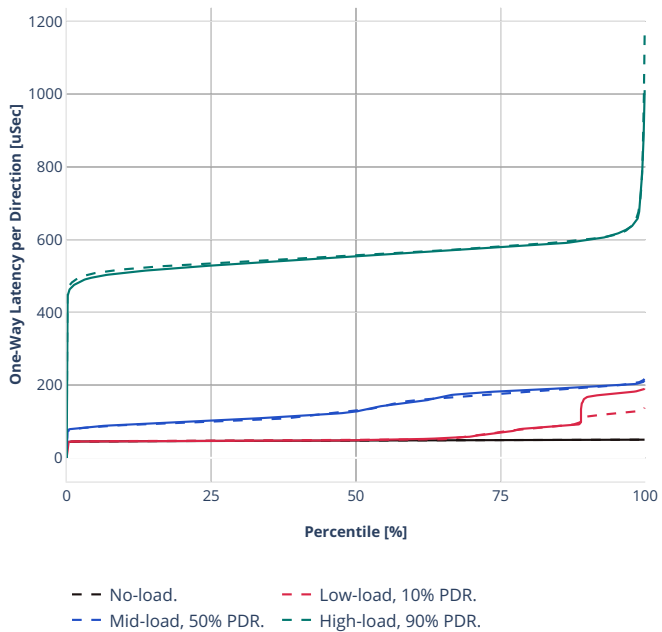
Latency: eth-l2bdbasemaclrn-eth-2memif-1lxc
