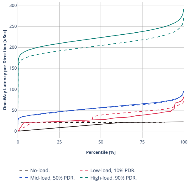
Latency: eth-l2xcbase-eth-2memif-1lxc
