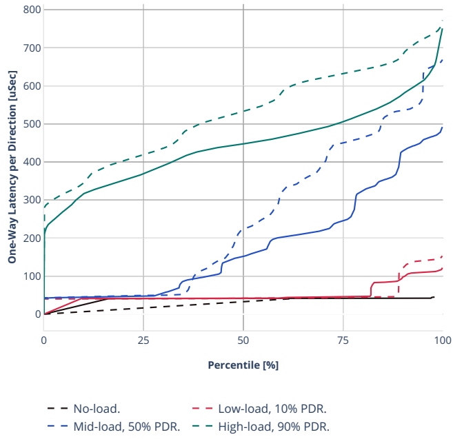
Latency: avf-ethip4ipsec1000tnlsw-ip4base-int-aes128cbc-hmac512sha
