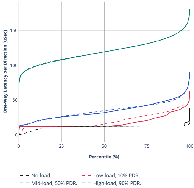
Latency: eth-l2bdbasemaclrn-eth-2vhostvr1024-1vm
