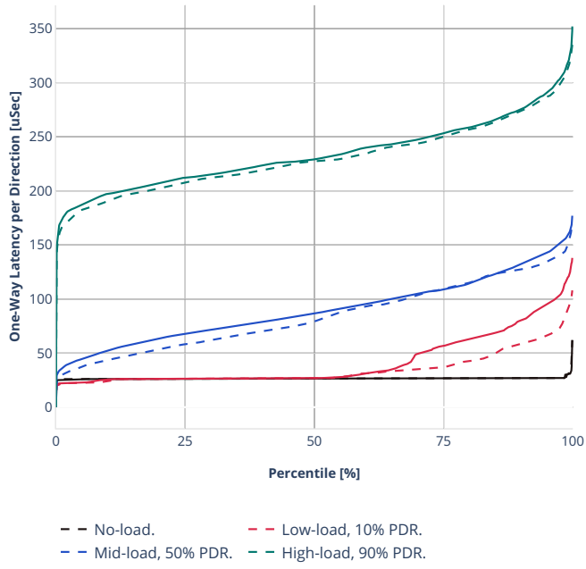
Latency: eth-l2bdbasemaclrn-eth-2vhostv1024-1vm
