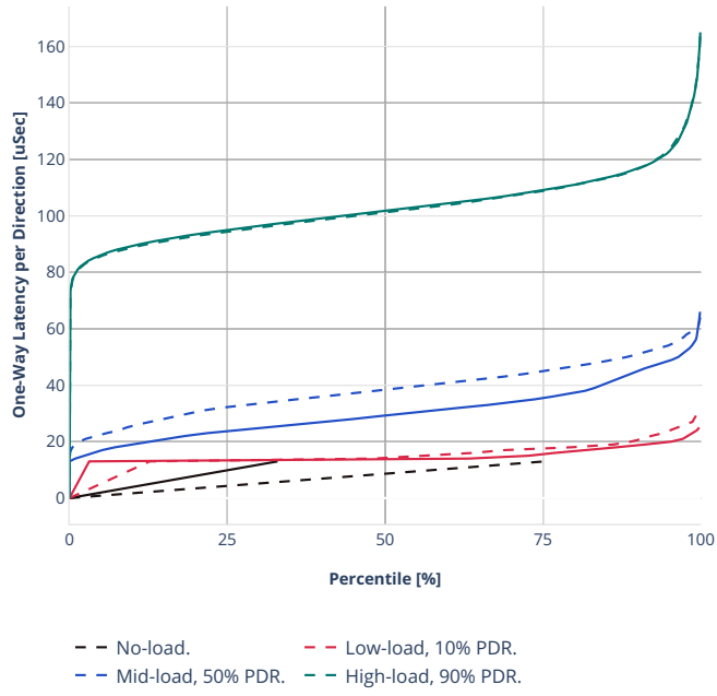
Latency: avf-ethip4-ip4base-eth-2memif-1dcr
