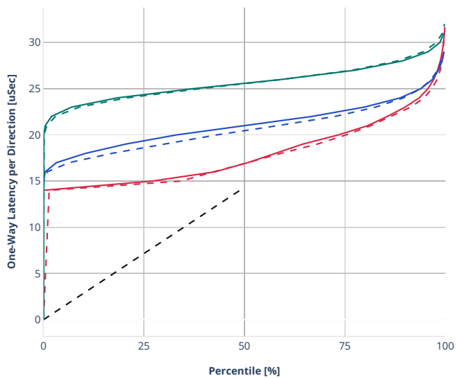
Latency: avf-eth-l2patch
