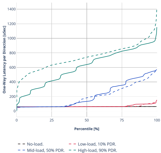
Latency: ethip4ipsec1000tnlhw-ip4base-int-aes128cbc-hmac512sha
