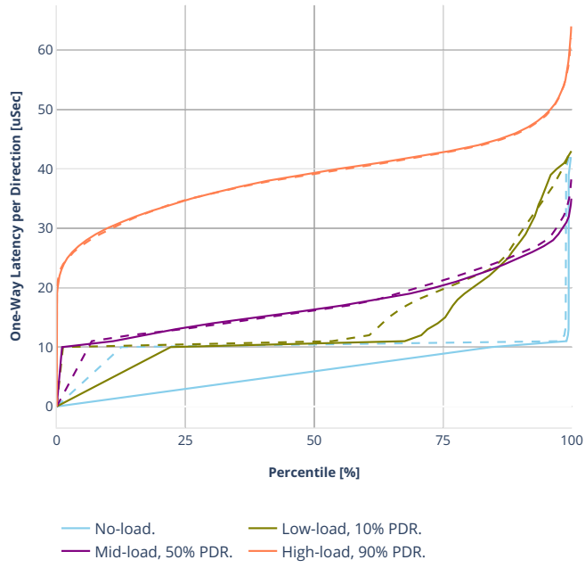
Latency: ethip4-ip4scale200k
