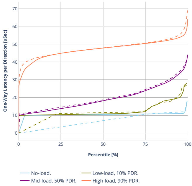
Latency: avf-ethip4udp-ip4scale1000-udpsrcscale15-nat44
