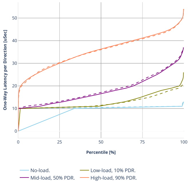
Latency: avf-ethip4udp-ip4base-oac150sl-10kflows
