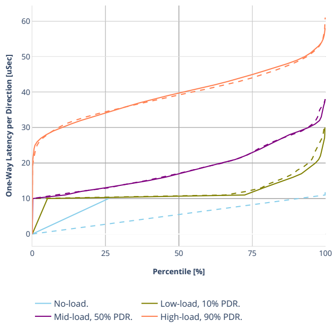
Latency: avf-ethip4udp-ip4base-nat44
