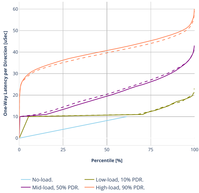
Latency: avf-ethip4udp-ip4base-nat44
