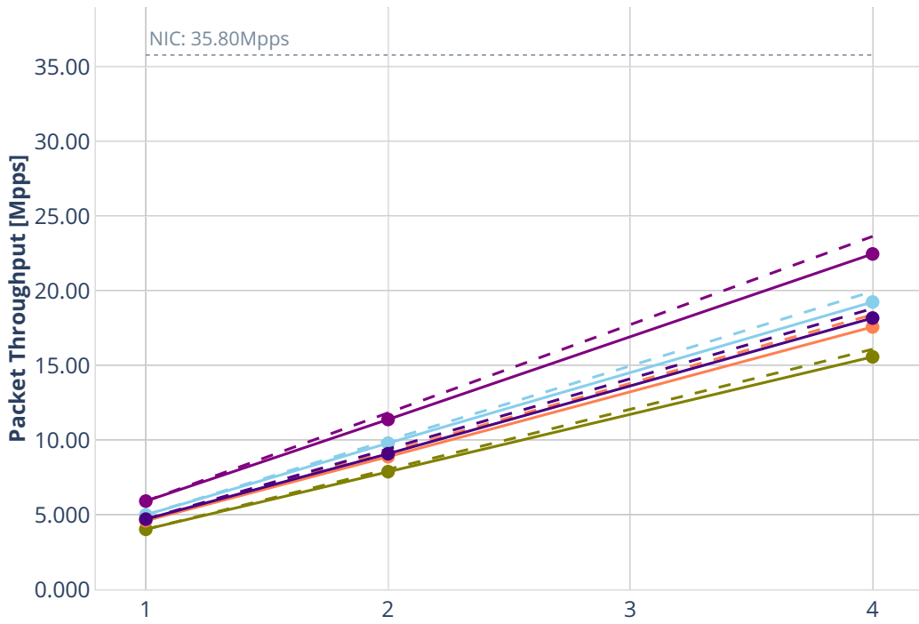
Number of Cores [Qty] --- Perfect — Measured ... Limit dot1q-l2xcbase-eth-2vhostvr1024-1vm dot1q-l2bdbasemaclrn-eth-2vhostvr1024-1vm eth-l2xcbase-eth-2vhostvr1024-1vm eth-l2bdbasemaclrn-eth-2vhostvr1024-1vm ethip4-ip4base-eth-2vhostvr1024-1vm
