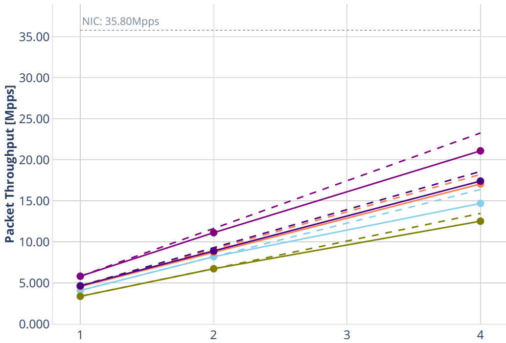
Number of Cores [Qty] -- Perfect — Measured ... Limit dot1q-l2xcbase-eth-2vhostvr1024-1vm dot1q-l2bdbasemaclrn-eth-2vhostvr1024-1vm eth-l2xcbase-eth-2vhostvr1024-1vm eth-l2bdbasemaclrn-eth-2vhostvr1024-1vm ethip4-ip4base-eth-2vhostvr1024-1vm
