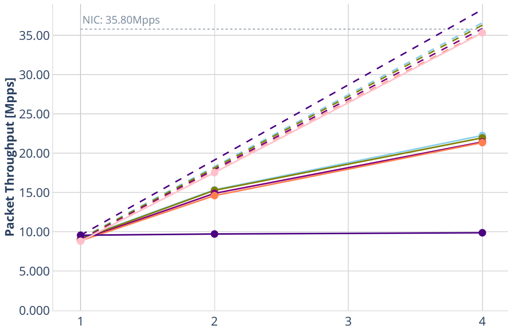
Number of Cores [Qty] --- Perfect — Measured ... Limit avf-ethip4udp-ip4base-iac150sf-10kflows avf-ethip4udp-ip4base-iac150sl-10kflows avf-ethip4udp-ip4base-oacl50sf-10kflows avf-ethip4udp-ip4base-oacl50sl-10kflows avf-ethip4udp-ip4base-nat44 avf-ethip4udp-ip4scale1000-udpsrcscale15-nat44
