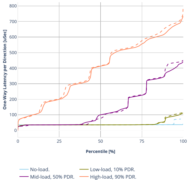
Latency: ethip4ipsec4tnlsw-ip4base-int-aes256gcm
