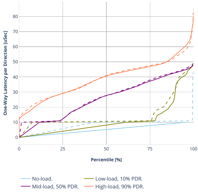
Latency: ethip6-ip6scale20k
