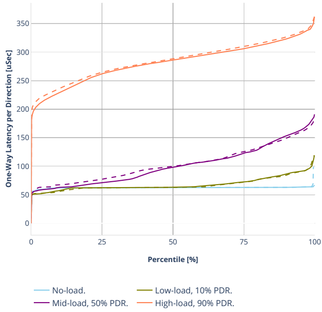
Latency: ethip4ipsec1000tnlhw-ip4base-int-aes128cbc-hmac512sha
