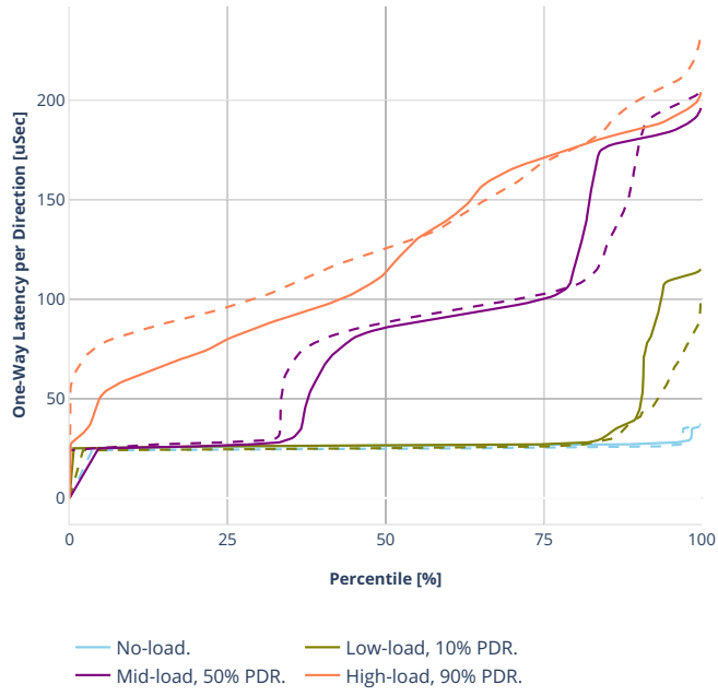
Latency: eth-l2bdbasemaclrn-oacl50sf-10kflows
