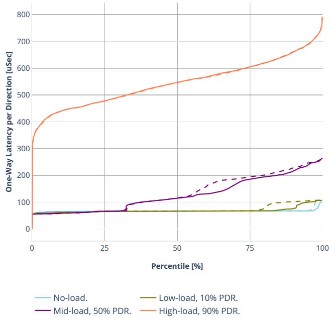
Latency: ethip4ipsec10000tnlsw-ip4base-int-aes128cbc-hmac512sha
