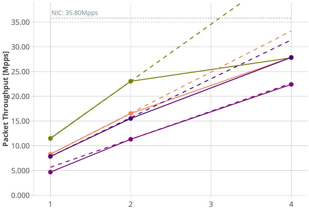
Number of Cores [Qty] --- Perfect — Measured ... Limit eth-l2xcbase-eth-2memif-1dcr eth-l2xcbase-eth-2memif-1xc dot1q-l2bdbasemaclrn-eth-2memif-1dcr eth-l2bdbasemaclrn-eth-2memif-1xc ethip4-ip4base-eth-2memif-1dcr
