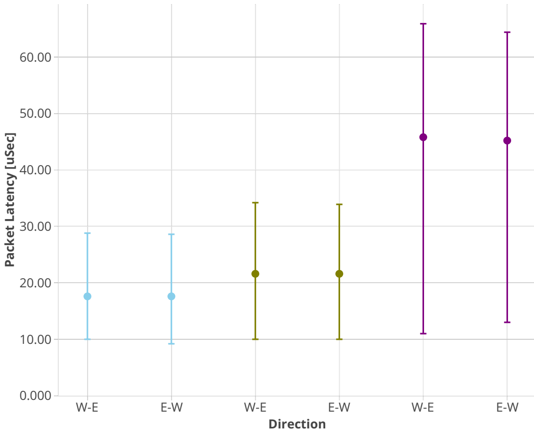
● avf-eth-l2patch ● avf-eth-l2xcbase ● avf-eth-l2bdbasemaclrn
