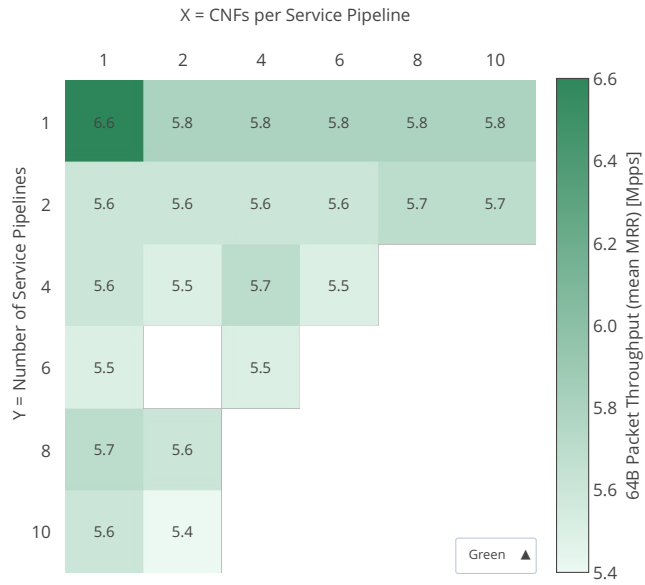
Throughput: eth-l2bd-{Y}pl-{2Y}mif-{XY}dcr-vppip4-mrr
