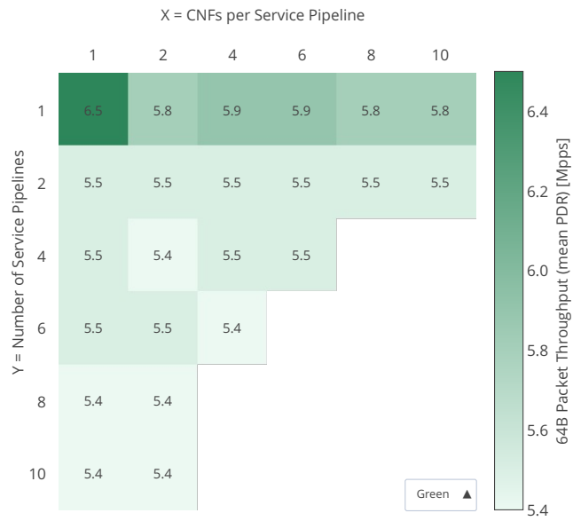
Throughput: eth-l2bd-{Y}pl-{2Y}mif-{XY}dcr-vppip4-pdr
