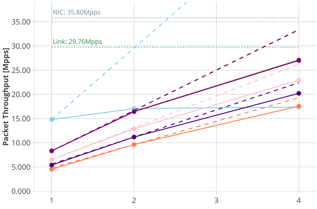
--- Perfect — Measured ... Limit eth-l2xcbase-eth-1memif-1dcr eth-l2xcbase-eth-2memif-1lxc eth-l2xcbase-eth-2memif-1dcr dot1q-l2bdbasemaclrn-eth-2memif-1dcr eth-l2bdbasemaclrn-eth-2memif-1lxc ethip4-ip4base-eth-2memif-1dcr
