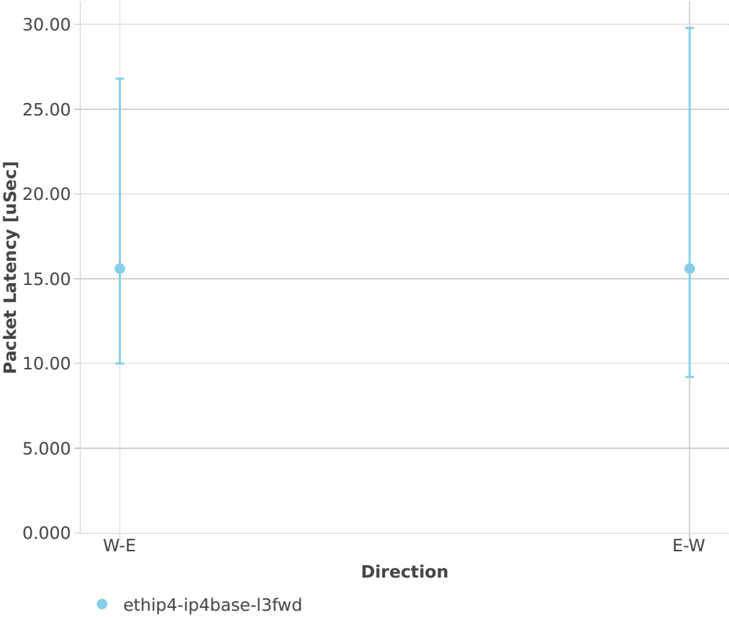
Latency: l3fwd-3n-skx-xxv710-64b-2t1c-base-ndr
