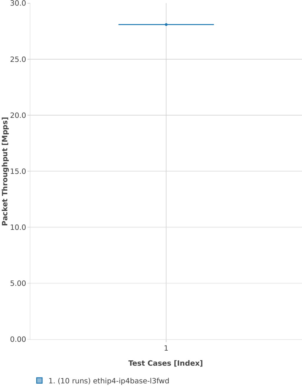
Throughput: l3fwd-3n-hsw-x710-64b-1t1c-base-pdr
