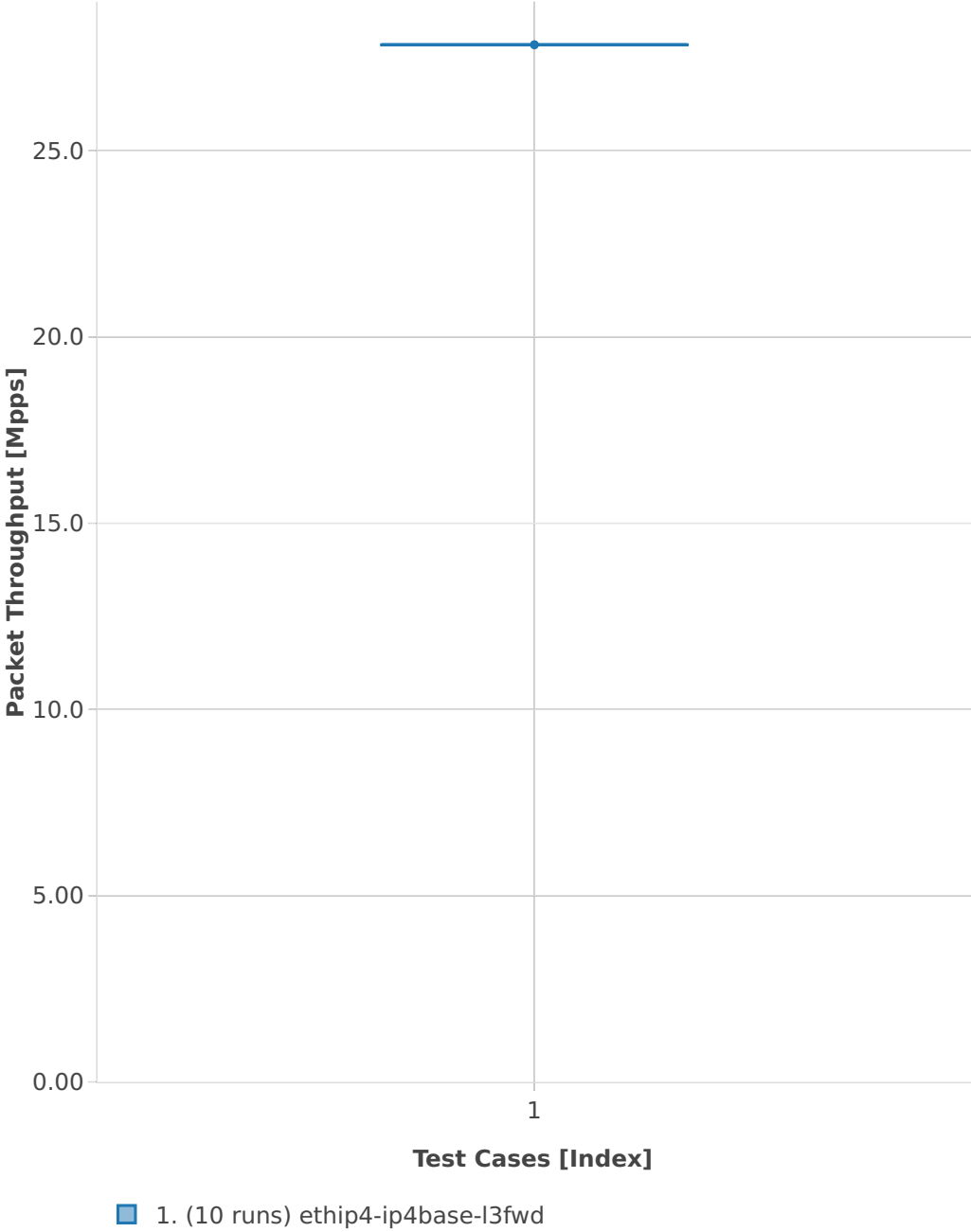
Throughput: l3fwd-3n-hsw-x520-64b-2t2c-base-ndr
