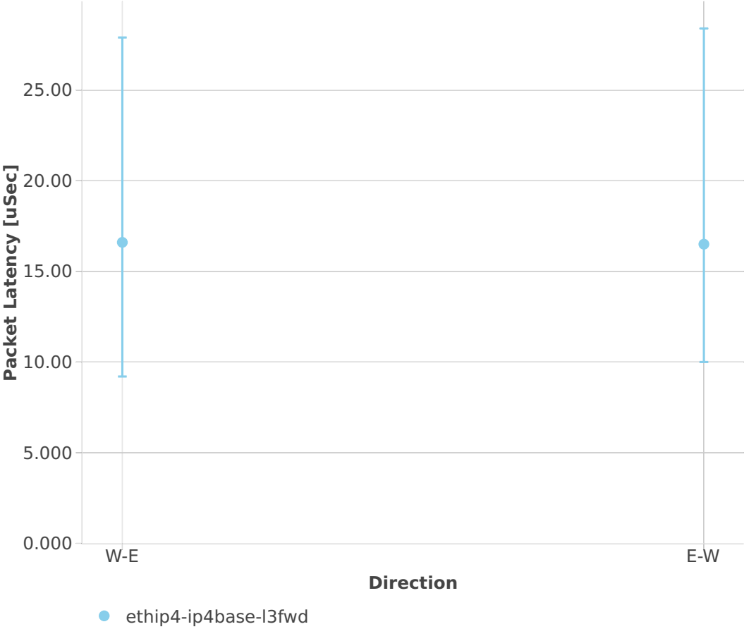
Latency: l3fwd-2n-skx-xxv710-64b-2t1c-base-ndr
