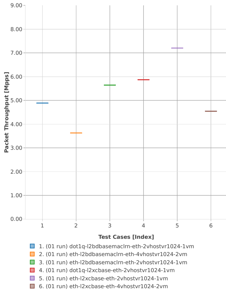
Throughput: vhost-l2sw-3n-skx-x710-64b-2t1c-base_and_features-vm-ndr
