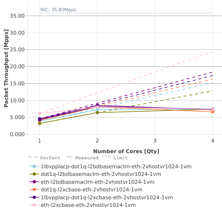
Speedup Multi-core: vhost-l2sw-3n-hsw-x710-64b-base_and_features-ndr
