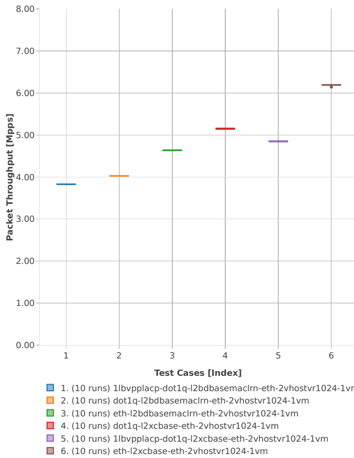
Throughput: vhost-l2sw-3n-hsw-x710-64b-1t1c-base_and_features-pdr
