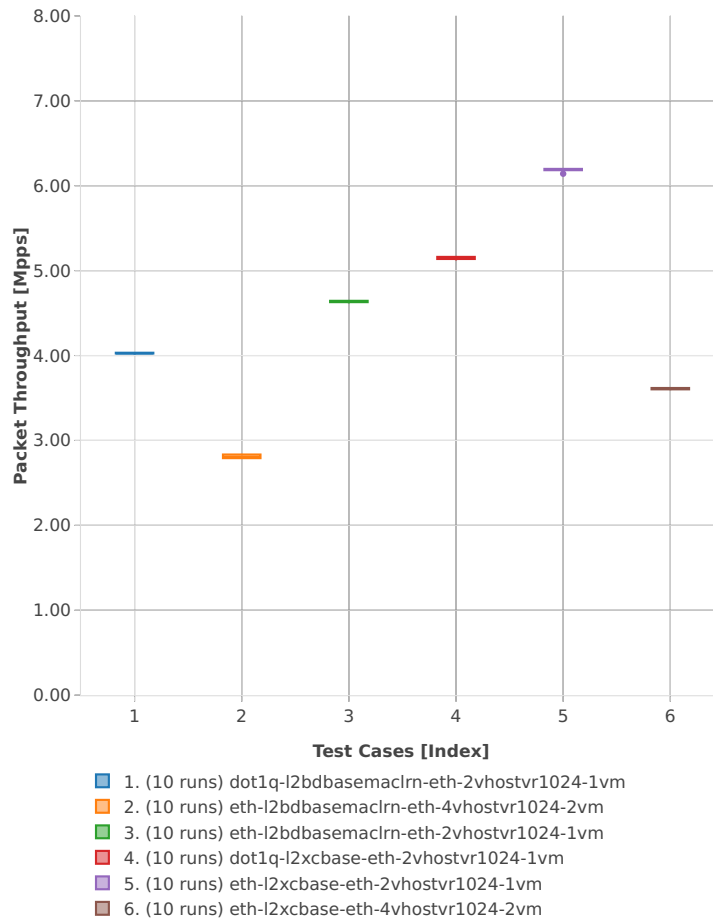
Throughput: vhost-l2sw-3n-hsw-x710-64b-1t1c-base_and_features-vm-pdr
