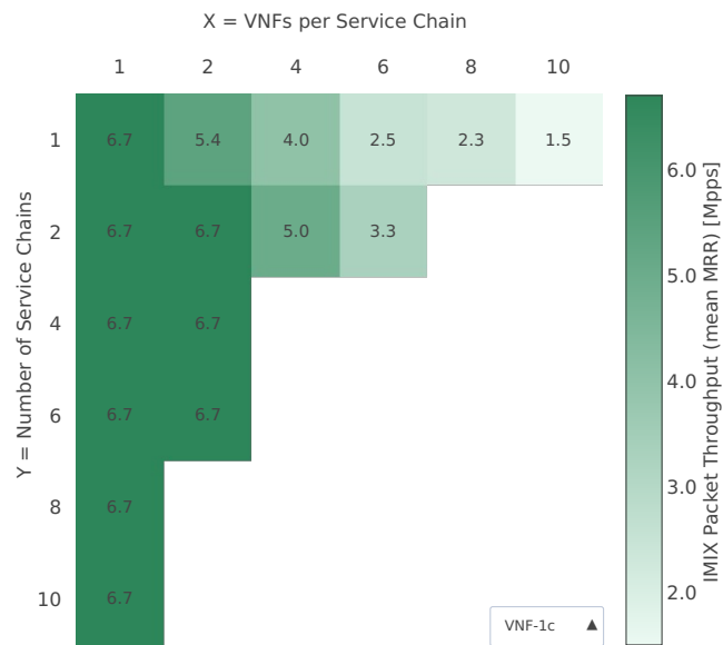
Throughput: eth-l2bd-{Y}ch-{2XY}vh-{XY}vm-vppip4-mrr
