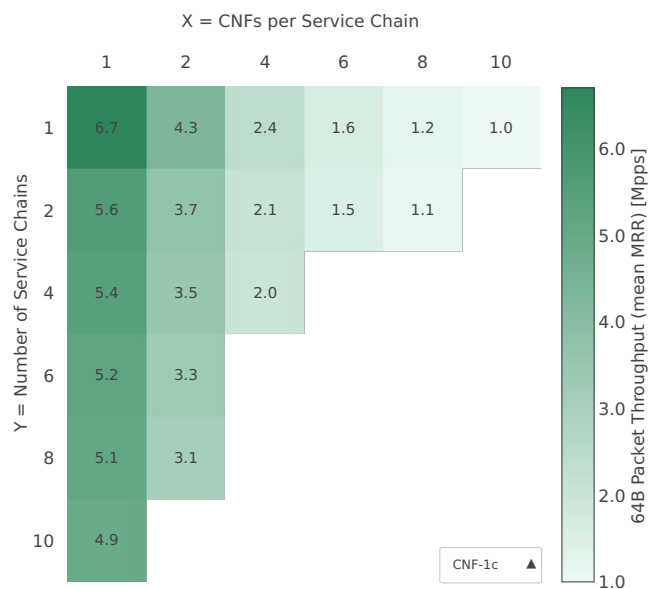
Throughput: eth-l2bd- \{Y\} ch- \{2XY\} mif- \{XY\} dcr-vppip4-mrr
