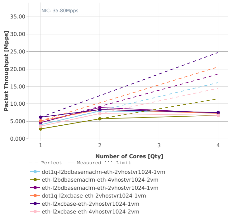
ipdup Multi-core: vhost-l2sw-3n-hsw-x710-64b-base_and_features-vm-pd
