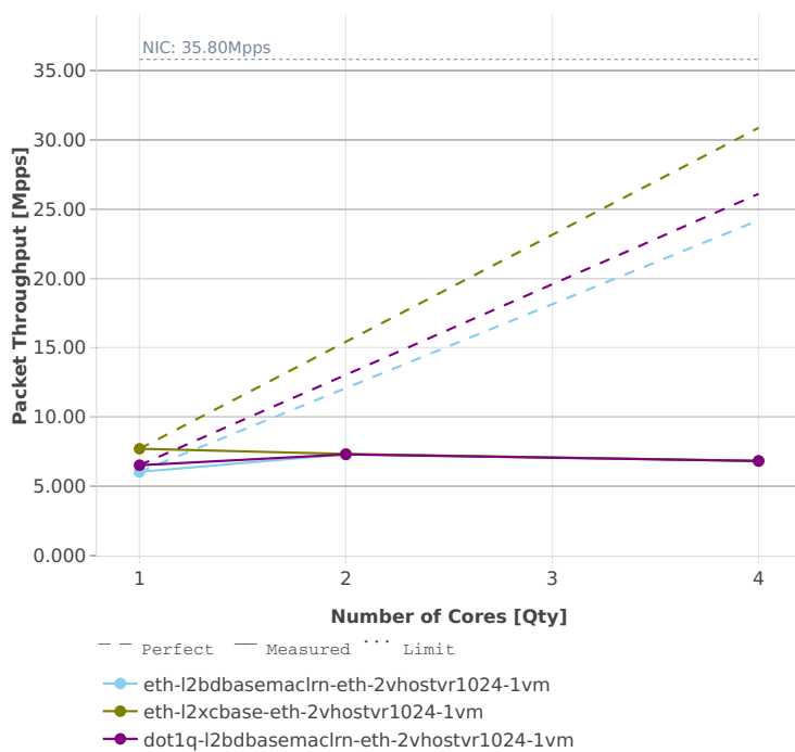
Speedup Multi-core: vhost-l2sw-2n-skx-x710-64b-base_and_features-pdr
