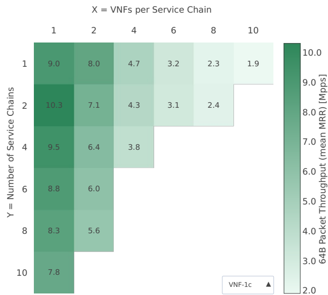
Throughput: eth-l2bd-{Y}ch-{2XY}vh-{XY}vm-vppip4-mrr
