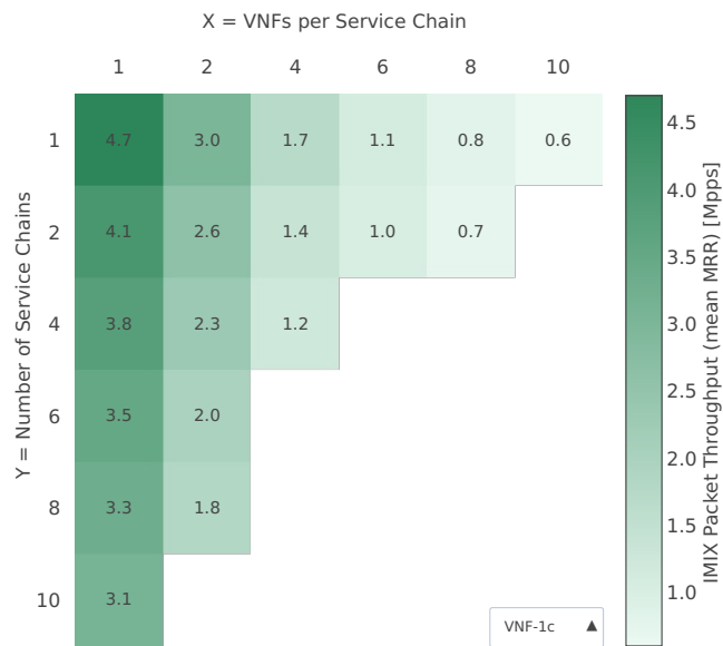
Throughput: eth-l2bd-{Y}ch-{2XY}vh-{XY}vm-vppip4-mrr
