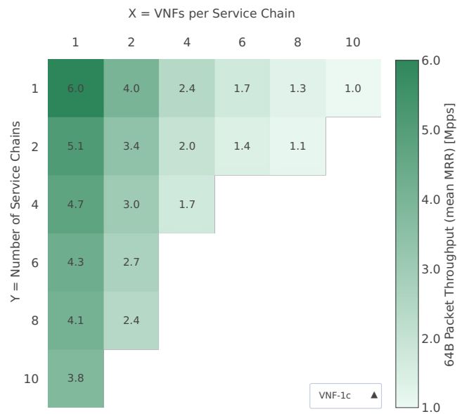
Throughput: eth-l2bd-{Y}ch-{2XY}vh-{XY}vm-vppip4-mrr
