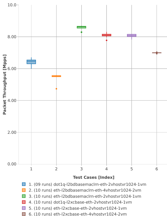
Throughput: vhost-l2sw-3n-hsw-x710-64b-2t2c-base_and_features-vm-ndr
