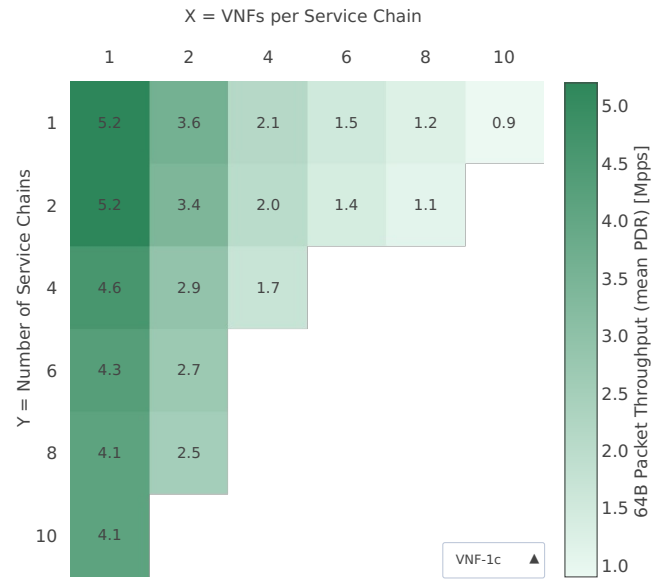
Throughput: eth-l2bd-{Y}ch-{2XY}vh-{XY}vm-vppip4-pdr
