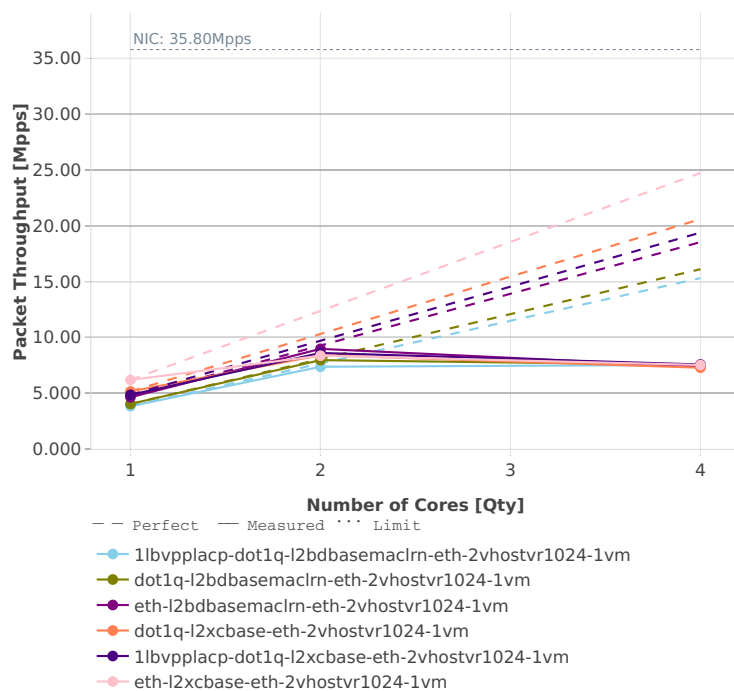
Speedup Multi-core: vhost-l2sw-3n-hsw-x710-64b-base_and_features-pdr
