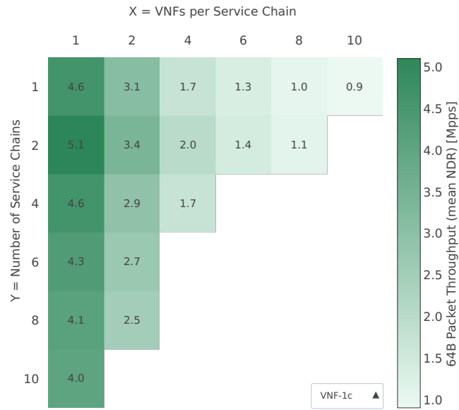
Throughput: eth-l2bd-{Y}ch-{2XY}vh-{XY}vm-vppip4-ndr
