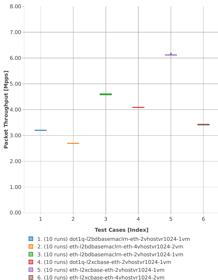
Throughput: vhost-l2sw-3n-hsw-x710-64b-1t1c-base_and_features-vm-ndr
