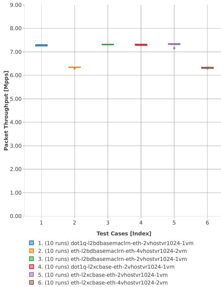
Throughput: vhost-l2sw-3n-skx-x710-64b-4t2c-base_and_features-vm-pdr
