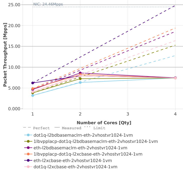
Speedup Multi-core: vhost-l2sw-3n-hsw-x520-64b-base_and_features-ndr
