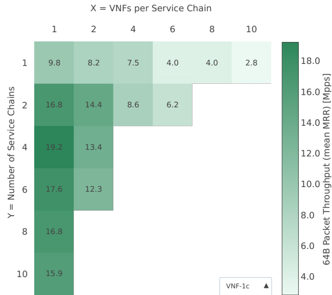
Throughput: eth-l2bd-{Y}ch-{2XY}vh-{XY}vm-vppip4-mrr
