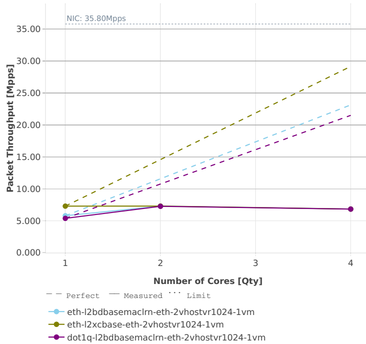
Speedup Multi-core: vhost-l2sw-2n-skx-x710-64b-base_and_features-ndr
