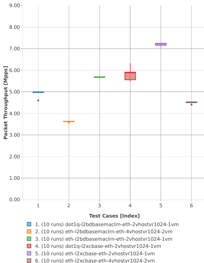
Throughput: vhost-l2sw-3n-skx-x710-64b-2t1c-base_and_features-vm-ndr
