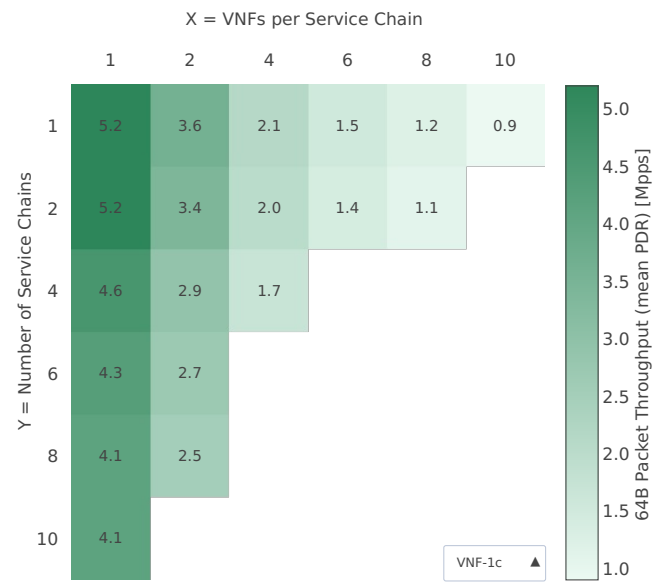
Throughput: eth-l2bd-{Y}ch-{2XY}vh-{XY}vm-vppip4-pdr
