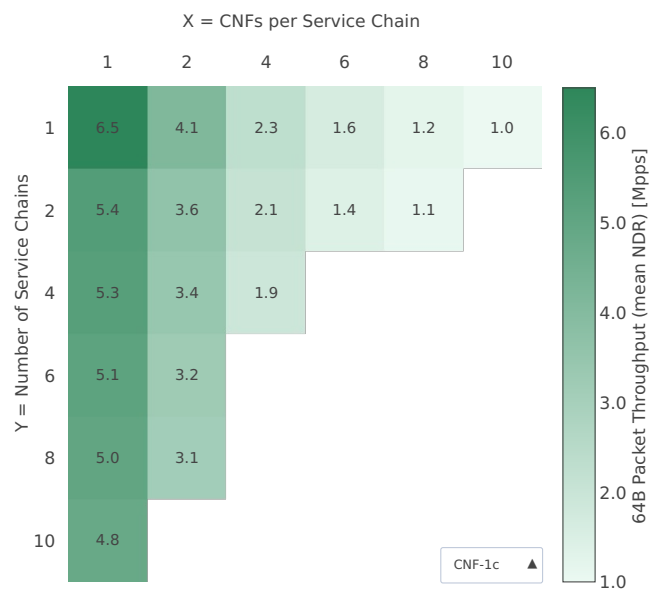
Throughput: eth-l2bd-{Y}ch-{2XY}mif-{XY}dcr-vppip4-ndr
