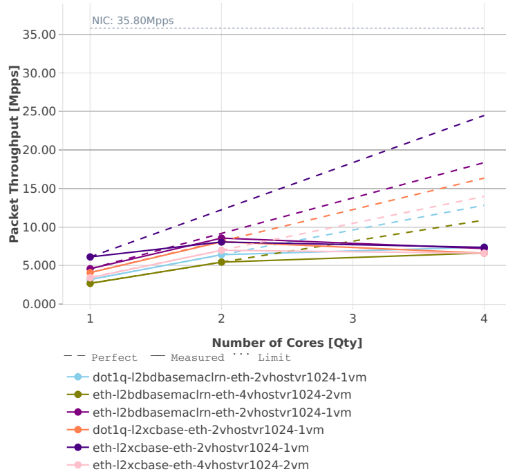
ipdup Multi-core: vhost-l2sw-3n-hsw-x710-64b-base_and_features-vm-nd
