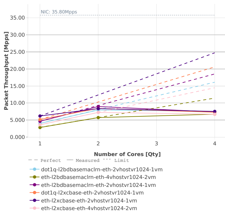
ipdup Multi-core: vhost-l2sw-3n-hsw-x710-64b-base_and_features-vm-pd
