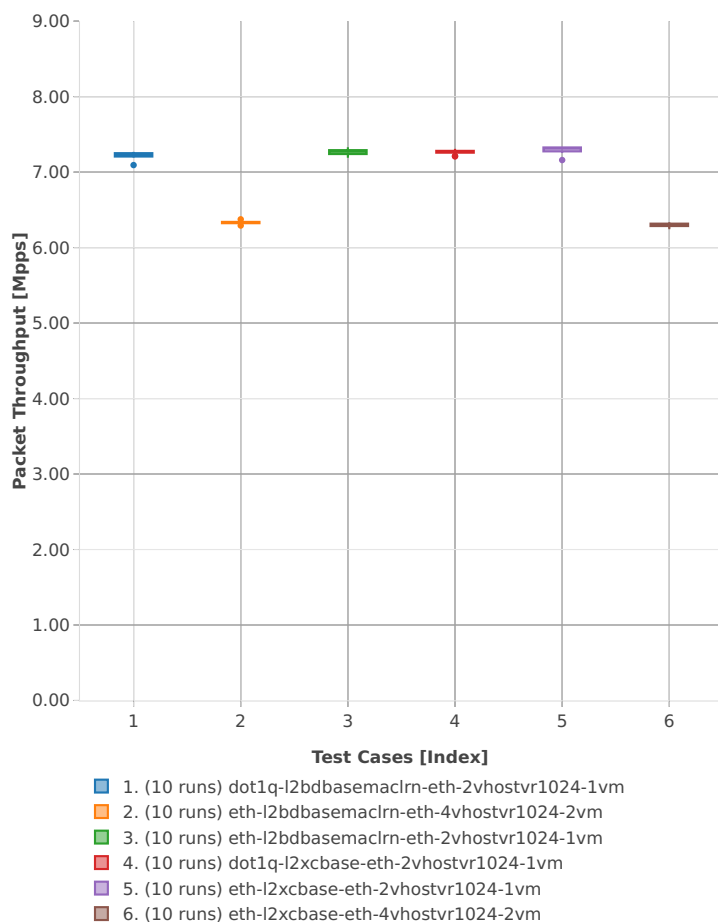
Throughput: vhost-l2sw-3n-skx-x710-64b-4t2c-base_and_features-vm-ndr
