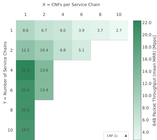
Throughput: eth-l2bd-{Y}ch-{2XY}mif-{XY}dcr-vppip4-mrr
