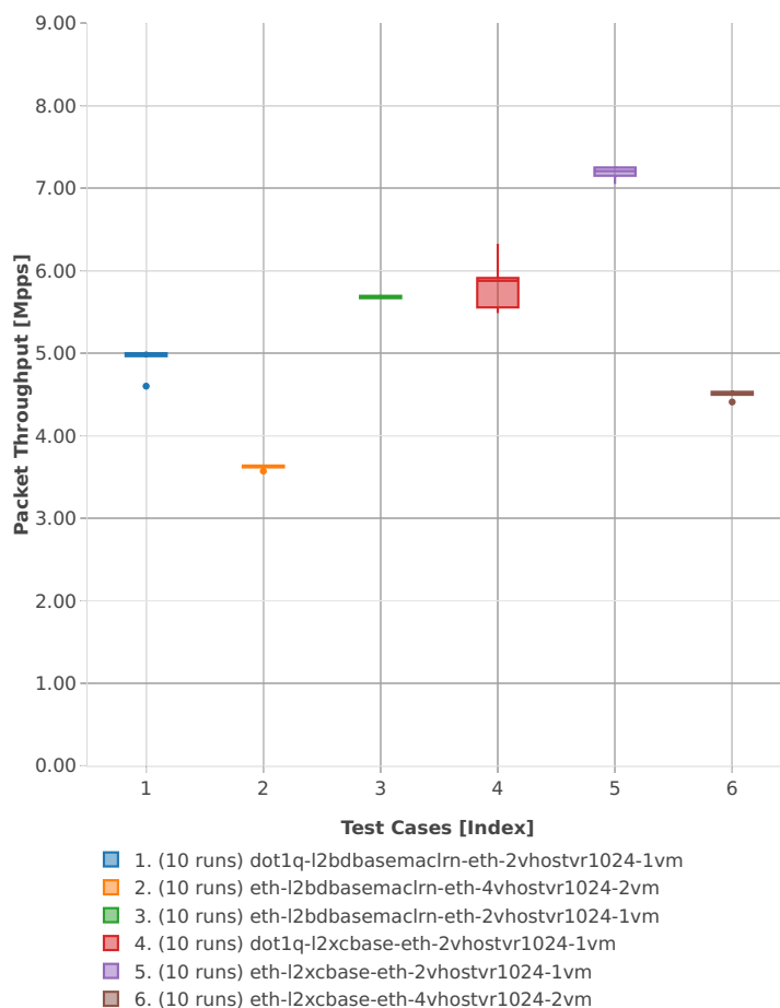
Throughput: vhost-l2sw-3n-skx-x710-64b-2t1c-base_and_features-vm-ndr
