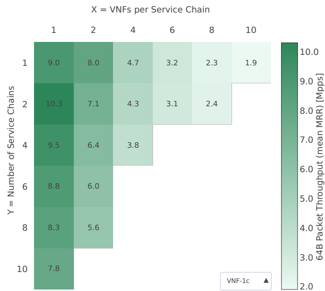
Throughput: eth-l2bd-{Y}ch-{2XY}vh-{XY}vm-vppip4-mrr
