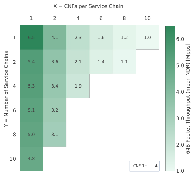
Throughput: eth-l2bd- \{Y\} ch- \{2XY\} mif- \{XY\} dcr-vppip4-ndr
