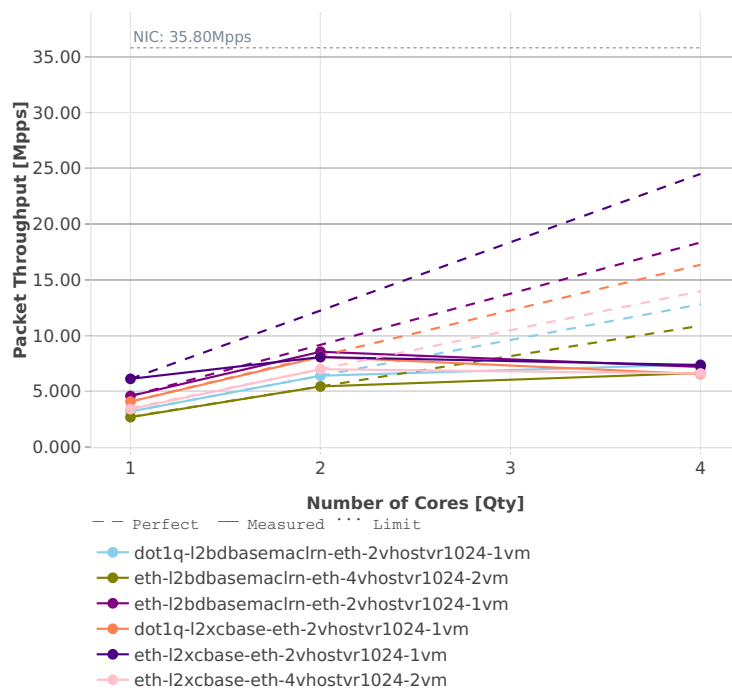
ipdup Multi-core: vhost-l2sw-3n-hsw-x710-64b-base_and_features-vm-nd
