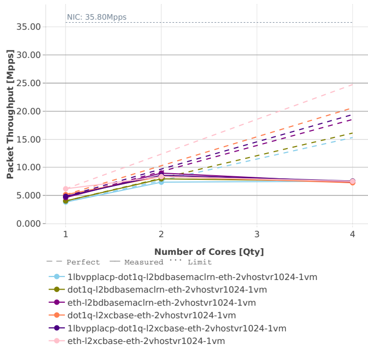
Speedup Multi-core: vhost-l2sw-3n-hsw-x710-64b-base_and_features-pdr
