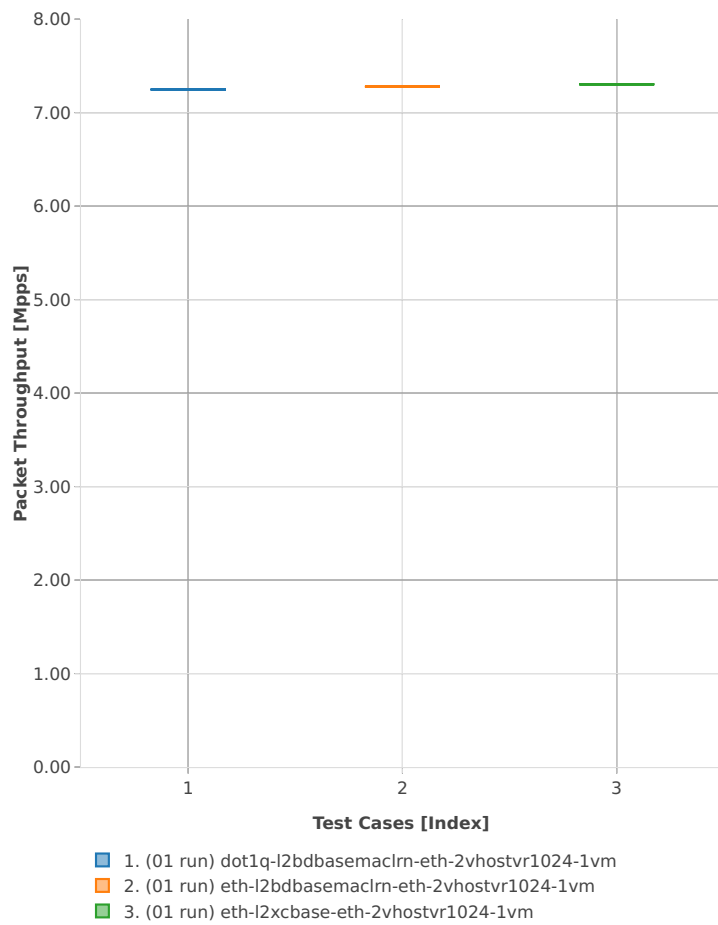
Throughput: vhost-l2sw-2n-skx-xxv710-64b-4t2c-base_and_features-ndr
