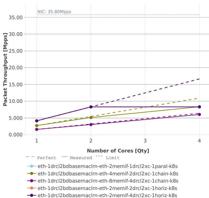
Speedup Multi-core: k8s-memif-3n-hsw-x710-64b-base_and_scale-l2bd-pdr
