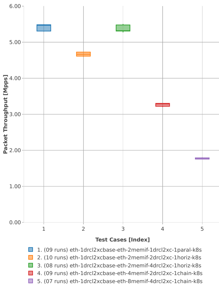
Throughput: k8s-memif-3n-hsw-x710-64b-1t1c-base_and_scale-l2xc-pdr
