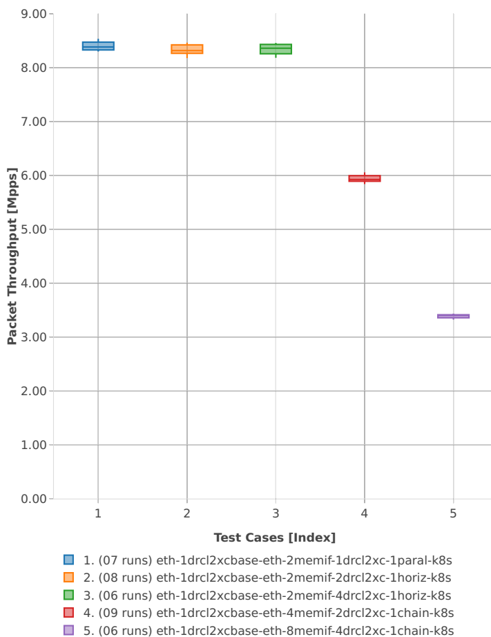
Throughput: k8s-memif-3n-hsw-x710-64b-2t2c-base_and_scale-l2xc-pdr
