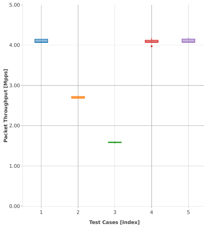
Throughput: k8s-memif-3n-hsw-x710-64b-1t1c-base_and_scale-l2bd-ndr
