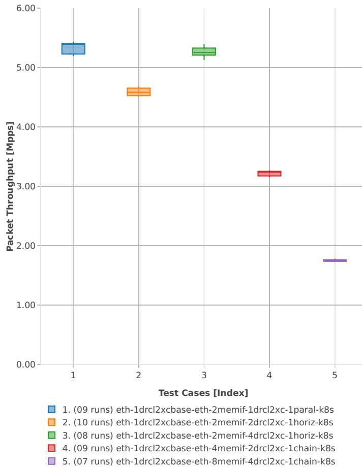
Throughput: k8s-memif-3n-hsw-x710-64b-1t1c-base_and_scale-l2xc-ndr
