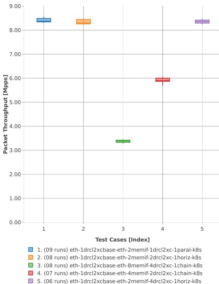
Throughput: k8s-memif-3n-hsw-x520-64b-2t2c-base_and_scale-l2xc-pdr
