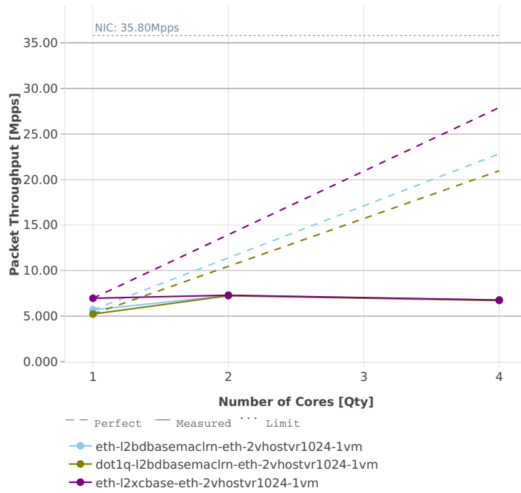
Speedup Multi-core: vhost-l2sw-2n-skx-xxv710-64b-base_and_features-pdr
