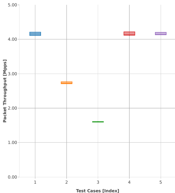
Throughput: k8s-memif-3n-hsw-x710-64b-1t1c-base_and_scale-l2bd-pdr
