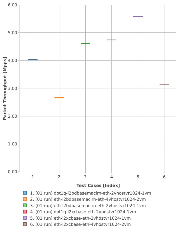
Throughput: vhost-l2sw-3n-hsw-x710-64b-1t1c-base_and_features-vm-pdr
