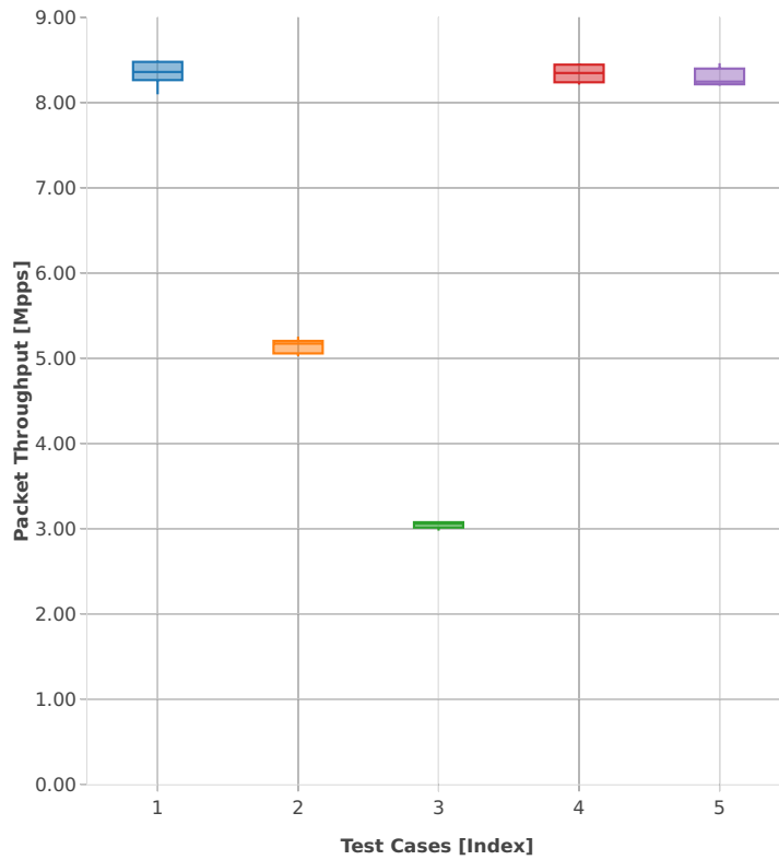
Throughput: k8s-memif-3n-hsw-x710-64b-2t2c-base_and_scale-l2bd-pdr
