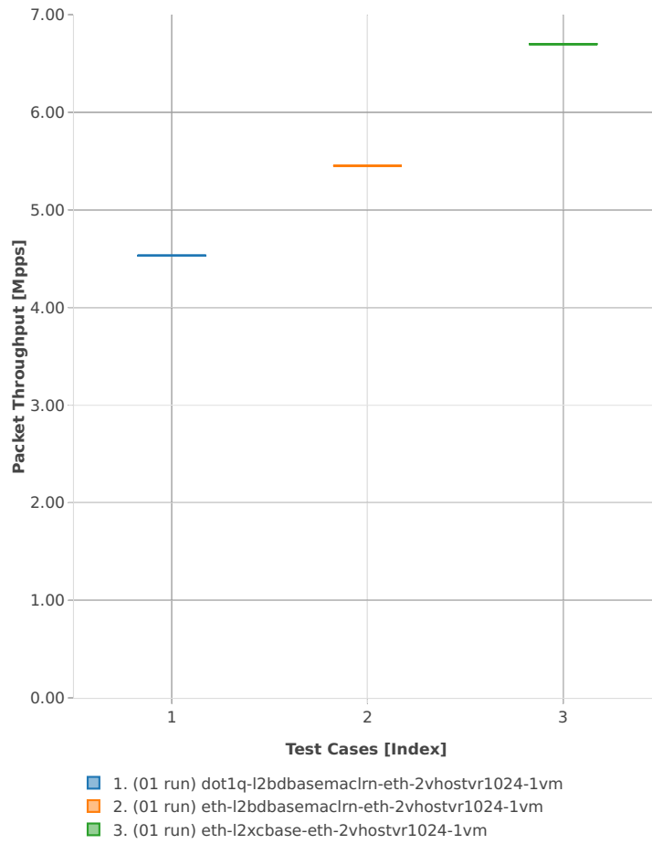
Throughput: vhost-l2sw-2n-skx-xxv710-64b-2t1c-base_and_features-ndr
