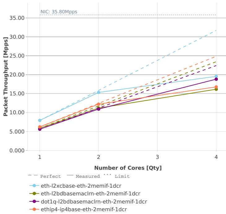
Speedup Multi-core: memif-2n-skx-xxv710-64b-base_and_features-pdr
