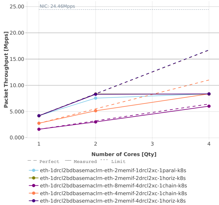
Speedup Multi-core: k8s-memif-3n-hsw-x520-64b-base_and_scale-l2bd-pdr
