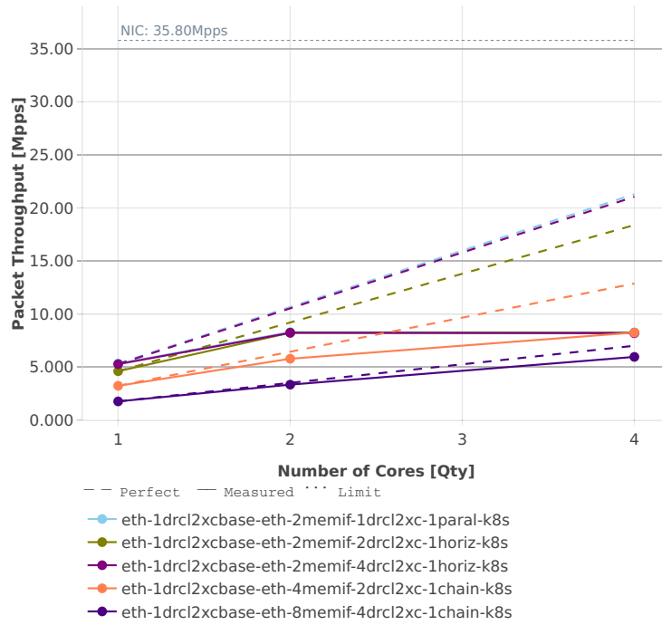
Speedup Multi-core: k8s-memif-3n-hsw-x710-64b-base_and_scale-l2xc-ndr
