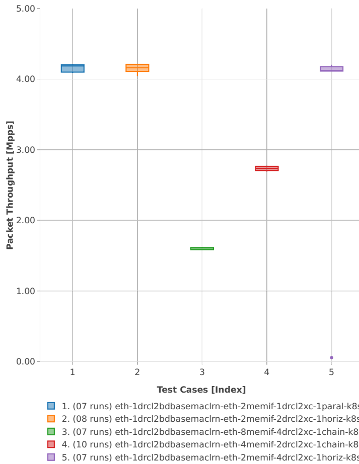
Throughput: k8s-memif-3n-hsw-x520-64b-1t1c-base_and_scale-l2bd-ndr
