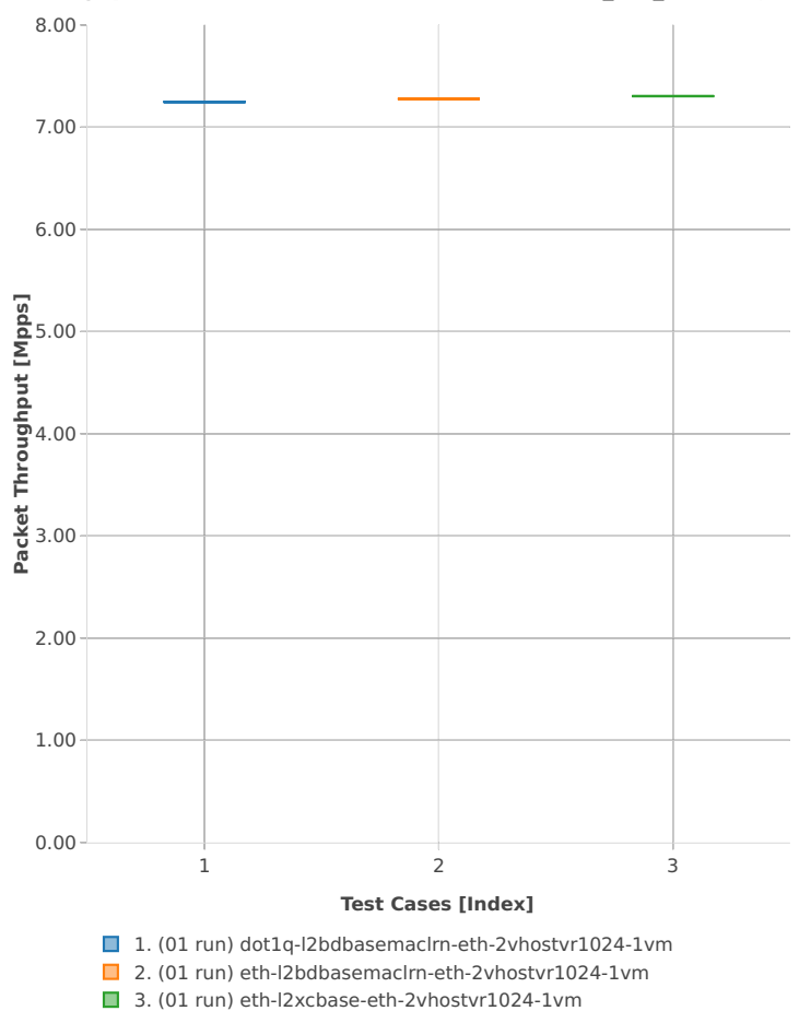
Throughput: vhost-l2sw-2n-skx-xxv710-64b-4t2c-base_and_features-pdr
