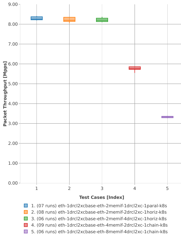
Throughput: k8s-memif-3n-hsw-x710-64b-2t2c-base_and_scale-l2xc-ndr
