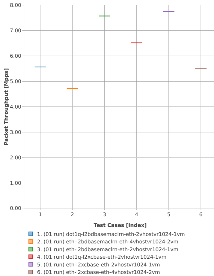
Throughput: vhost-l2sw-3n-hsw-x710-64b-2t2c-base_and_features-vm-ndr
