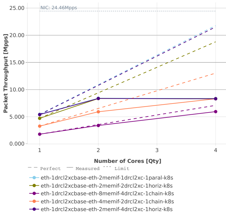
Speedup Multi-core: k8s-memif-3n-hsw-x520-64b-base_and_scale-l2xc-pdr
