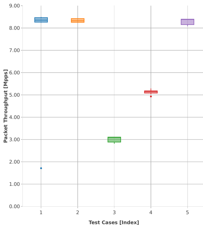
Throughput: k8s-memif-3n-hsw-x520-64b-2t2c-base_and_scale-l2bd-pdr
