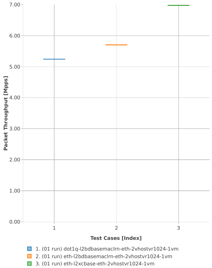
Throughput: vhost-l2sw-2n-skx-xxv710-64b-2t1c-base_and_features-pdr
