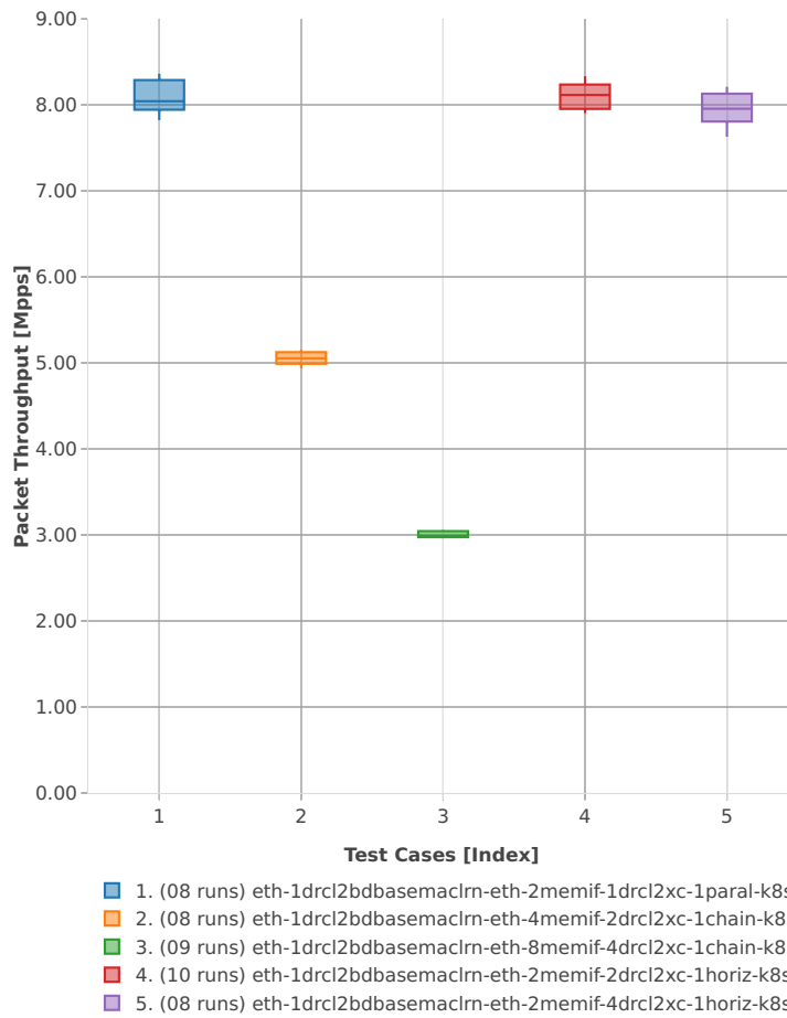
Throughput: k8s-memif-3n-hsw-x710-64b-2t2c-base_and_scale-l2bd-ndr
