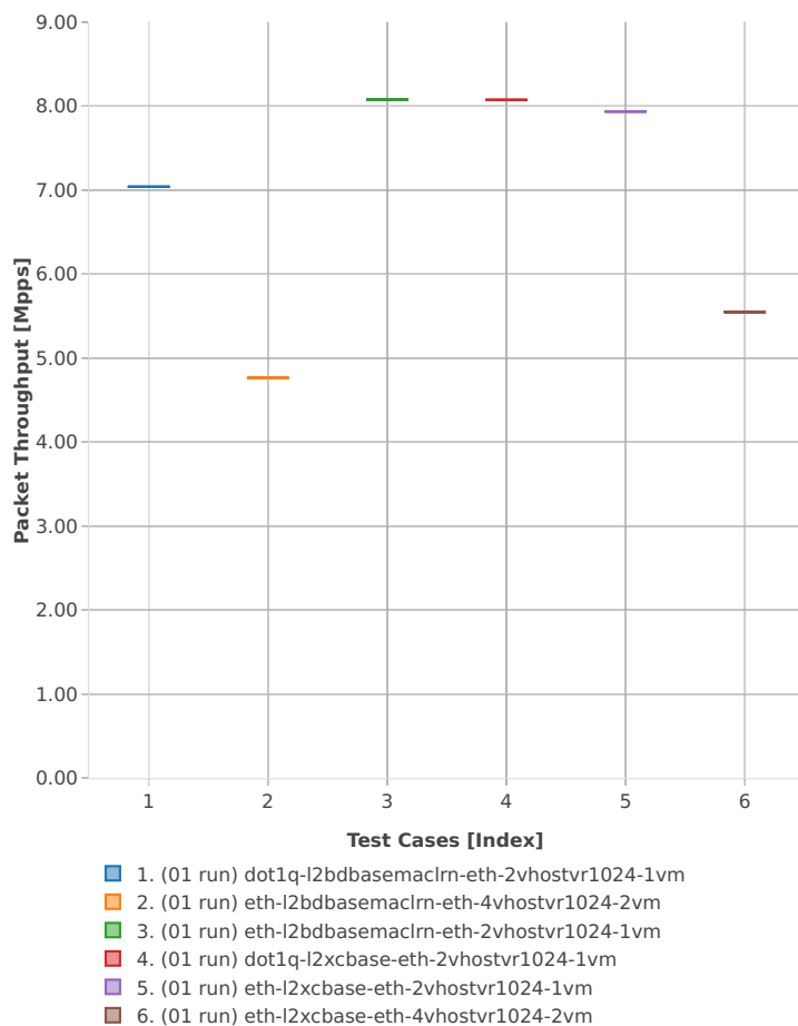
Throughput: vhost-l2sw-3n-hsw-x710-64b-2t2c-base_and_features-vm-pdr
