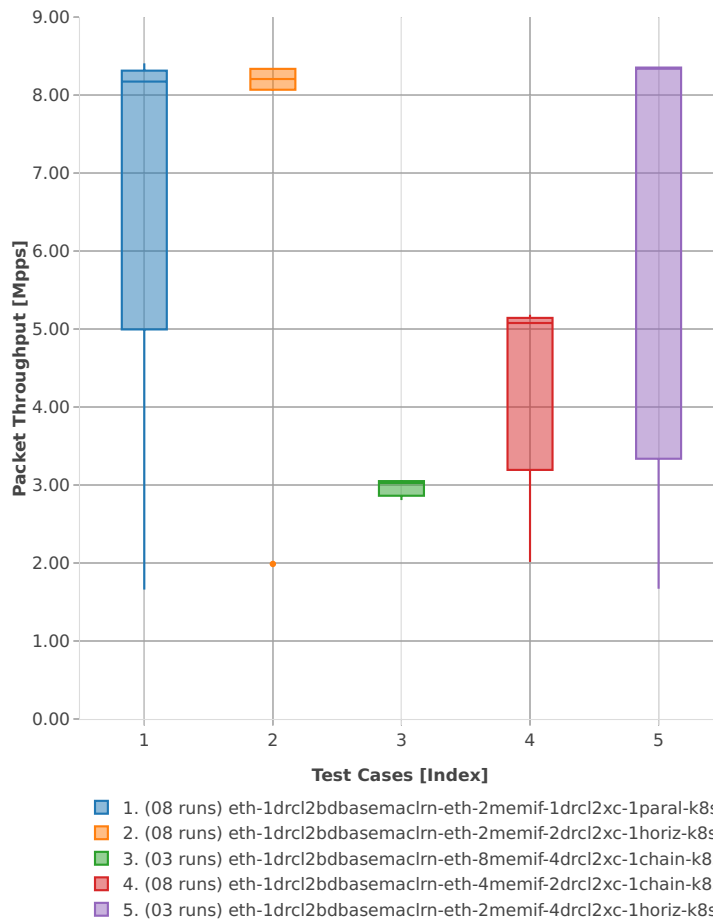
Throughput: k8s-memif-3n-hsw-x520-64b-2t2c-base_and_scale-l2bd-ndr
