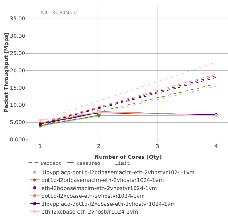
Speedup Multi-core: vhost-l2sw-3n-hsw-x710-64b-base_and_features-pdr
