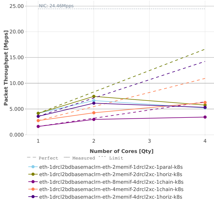
Speedup Multi-core: k8s-memif-3n-hsw-x520-64b-base_and_scale-ndr-l2bd
