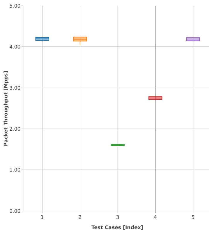
Throughput: k8s-memif-3n-hsw-x520-64b-1t1c-base_and_scale-l2bd-pdr
