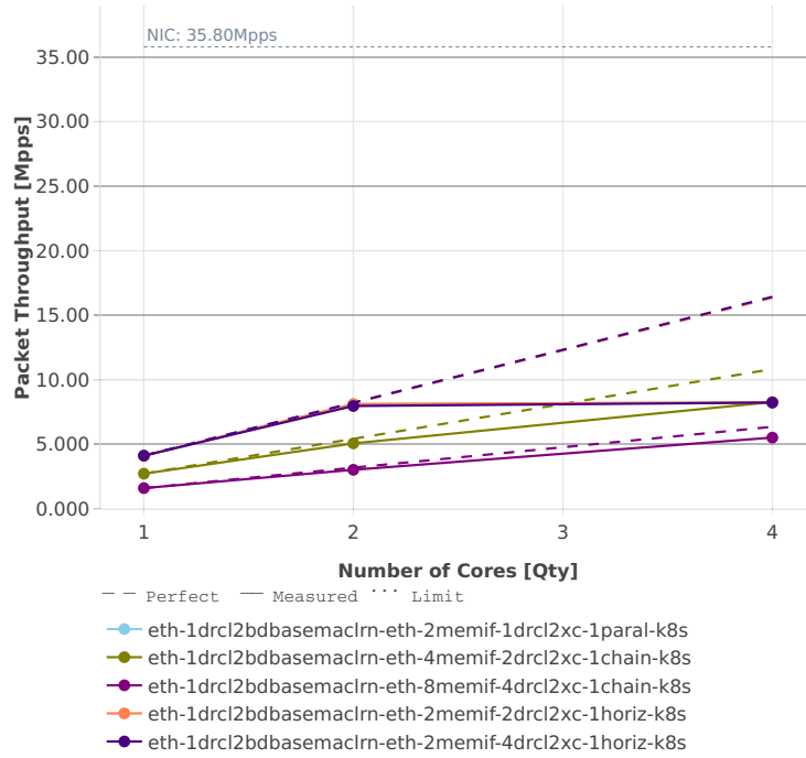
Speedup Multi-core: k8s-memif-3n-hsw-x710-64b-base_and_scale-l2bd-ndr
