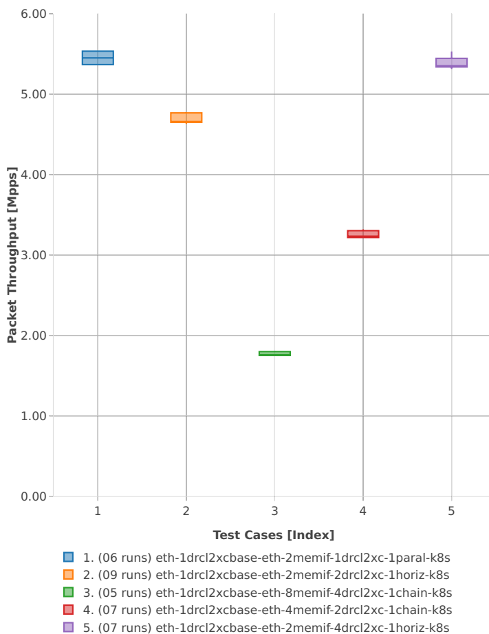
Throughput: k8s-memif-3n-hsw-x520-64b-1t1c-base_and_scale-l2xc-pdr
