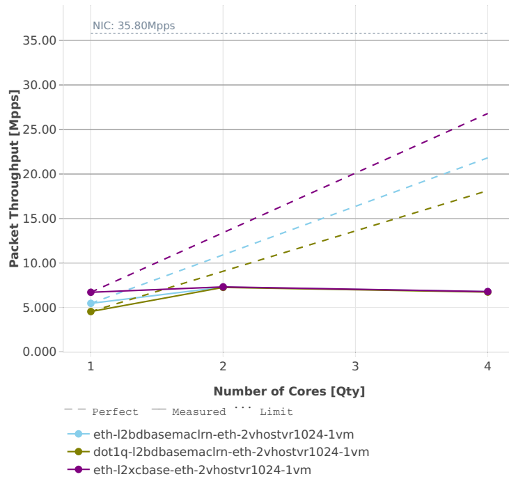
Speedup Multi-core: vhost-l2sw-2n-skx-xxv710-64b-base_and_features-ndr
