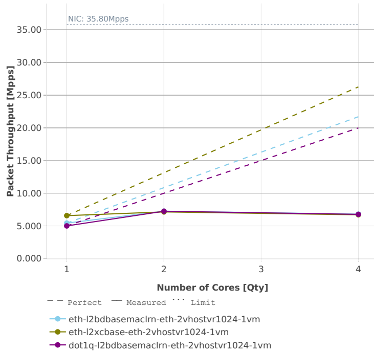
Speedup Multi-core: vhost-l2sw-2n-skx-x710-64b-base_and_features-ndr
