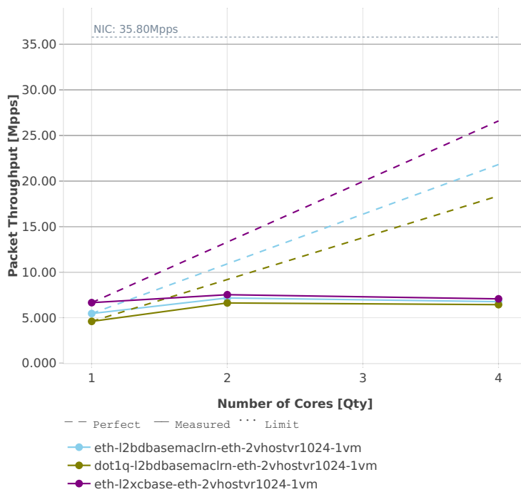
Speedup Multi-core: vhost-l2sw-2n-skx-xxv710-64b-base_and_features-ndr
