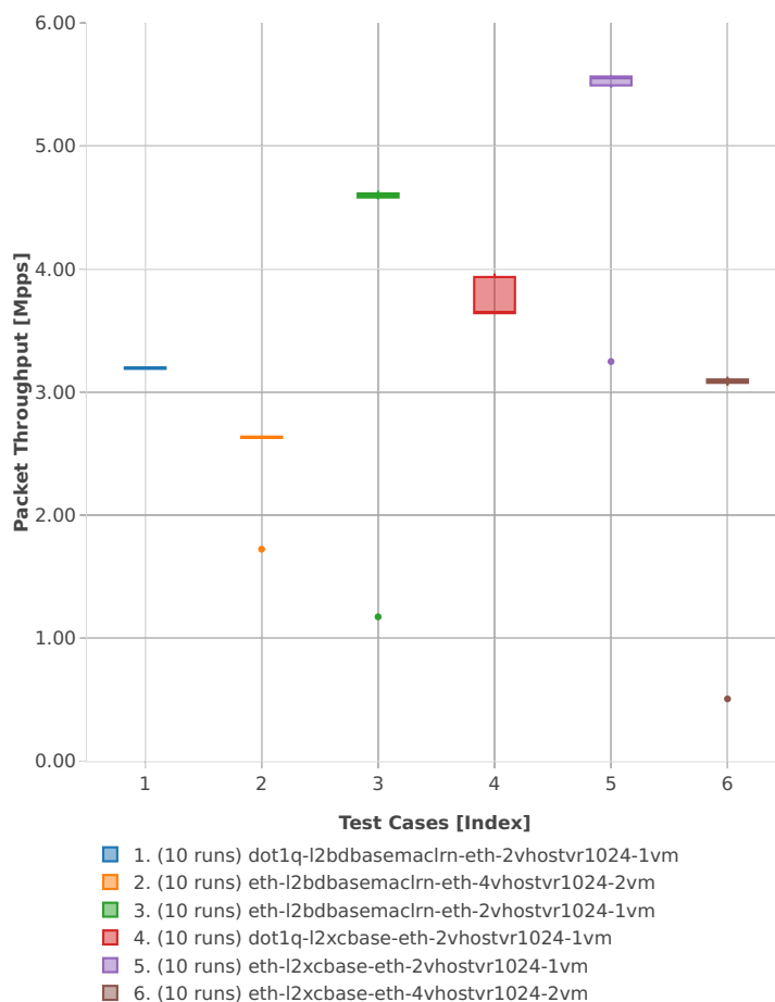
Throughput: vhost-l2sw-3n-hsw-x710-64b-1t1c-base_and_features-vm-ndr
