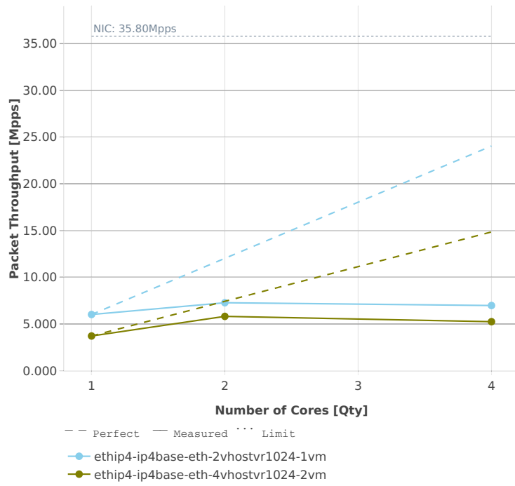
Speedup Multi-core: vhost-ip4-2n-skx-xxv710-64b-base_and_scale-pdr
