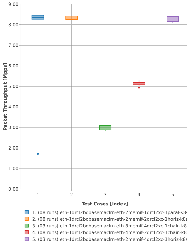
Throughput: k8s-memif-3n-hsw-x520-64b-2t2c-base_and_scale-l2bd-pdr
