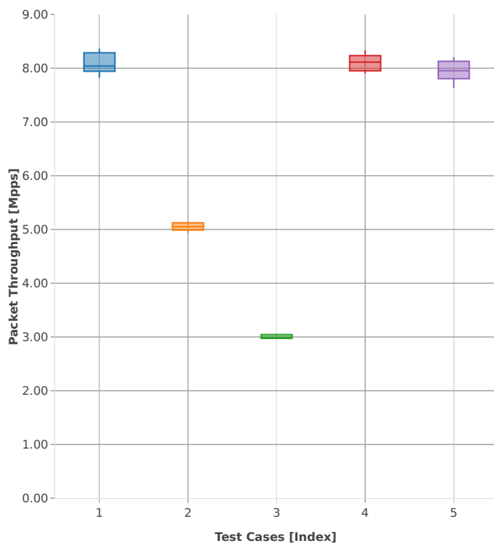
Throughput: k8s-memif-3n-hsw-x710-64b-2t2c-base_and_scale-l2bd-ndr
