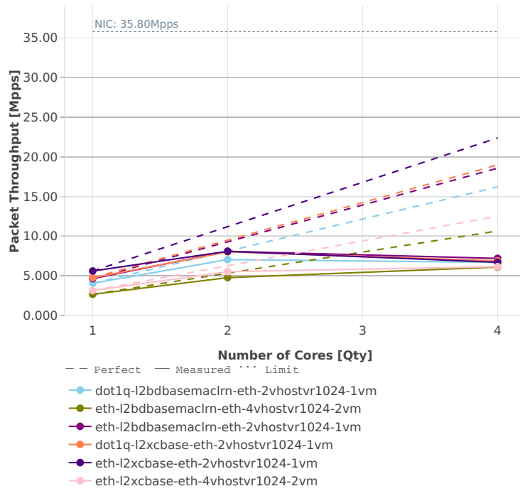
speedup Multi-core: vhost-l2sw-3n-hsw-x710-64b-base_and_features-vm-pd
