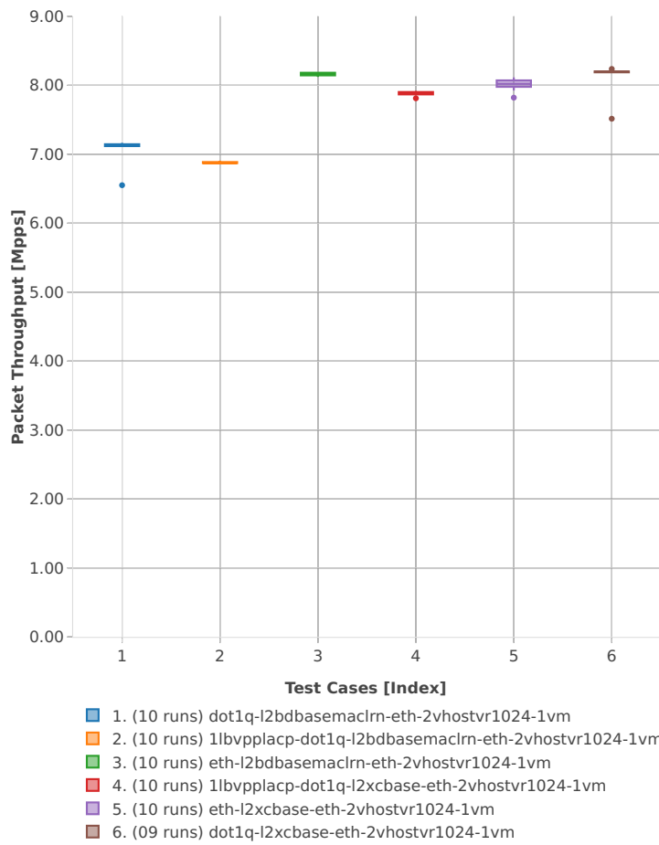
Throughput: vhost-l2sw-3n-hsw-x520-64b-2t2c-base_and_features-pdr
