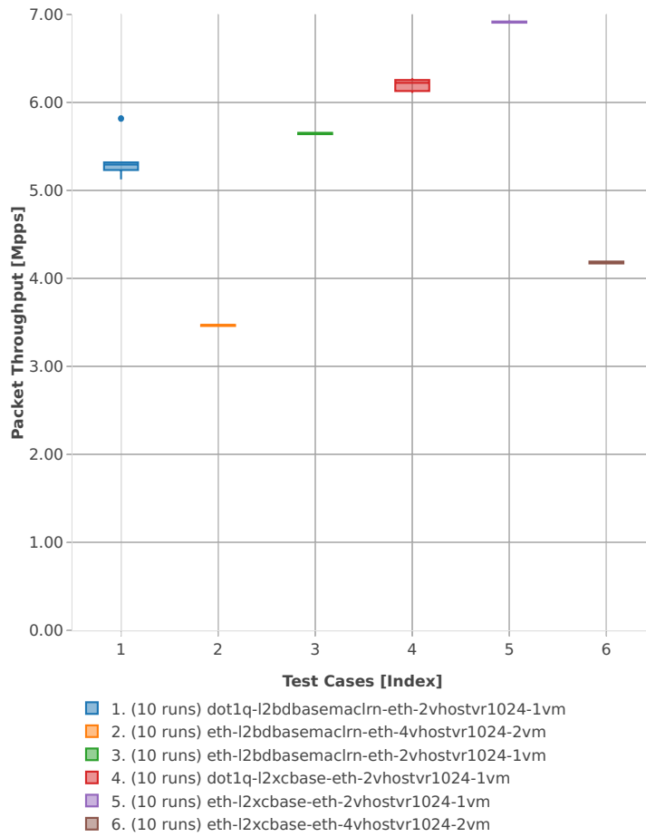
Throughput: vhost-l2sw-3n-skx-x710-64b-2t1c-base_and_features-vm-pdr
