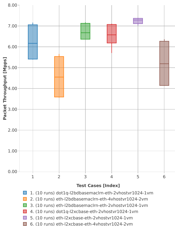
Throughput: vhost-l2sw-3n-skx-x710-64b-4t2c-base_and_features-vm-ndr
