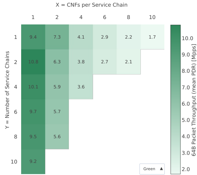
Throughput: eth-l2bd-{2XY}memif-{Y}chain-{XY}drc-vppip4-pdr
