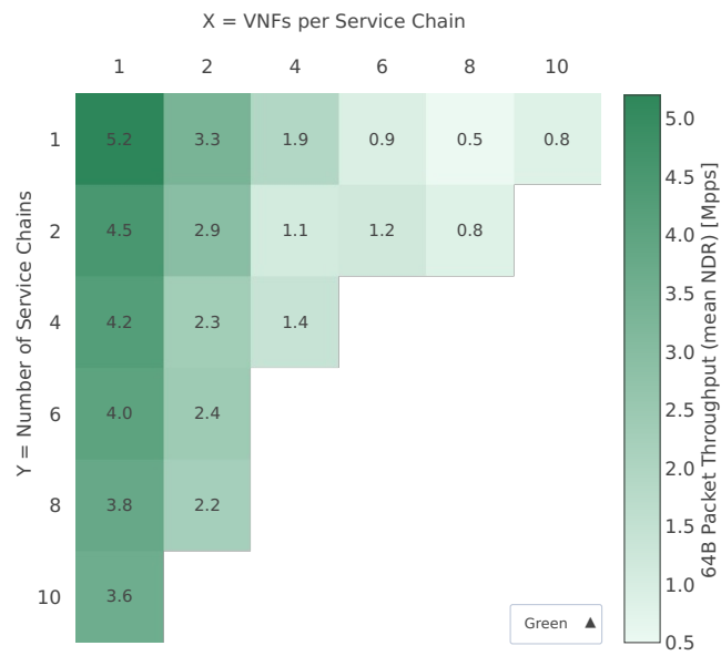
Throughput: eth-l2bd-{2XY}vhost-{Y}chain-{XY}vm-l3fwdip4-ndr
