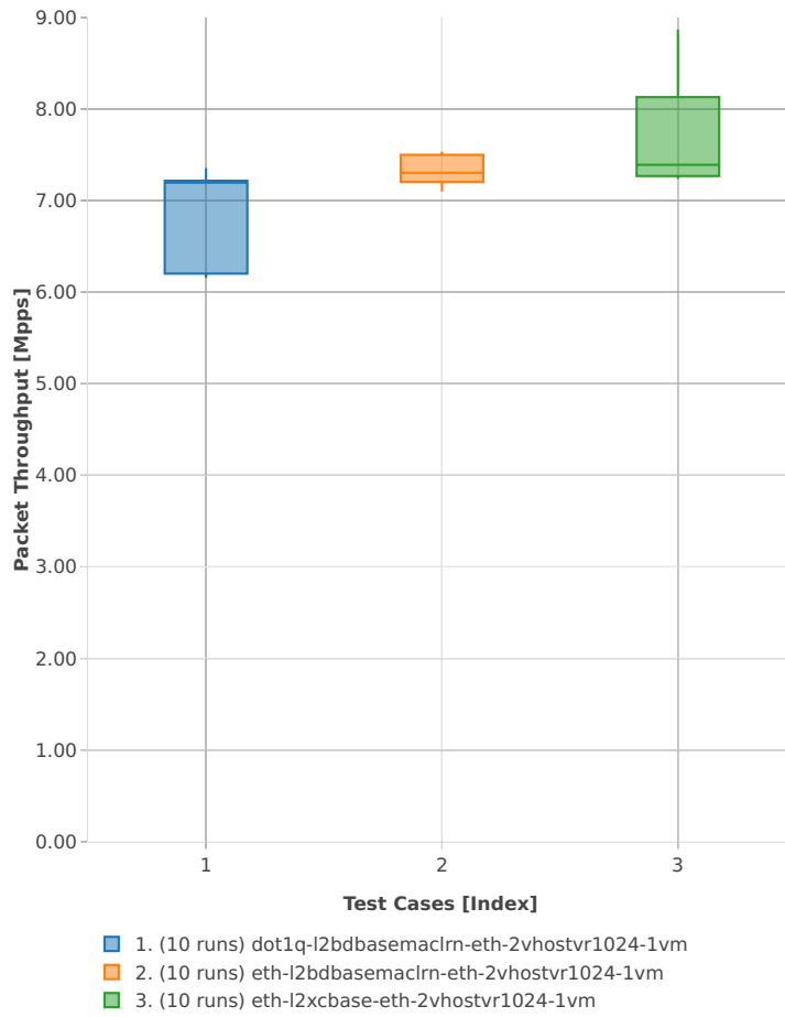
Throughput: vhost-l2sw-2n-skx-xxv710-64b-4t2c-base_and_features-pdr
