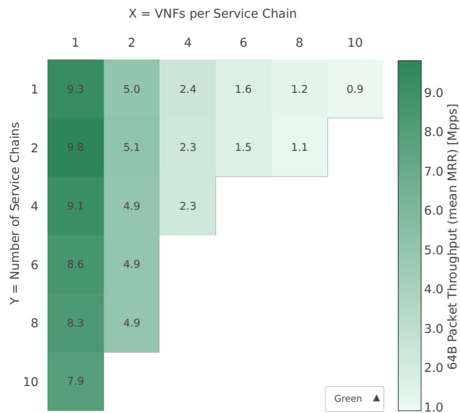
Throughput: eth-l2bd-{2XY}vhost-{Y}chain-{XY}vm-l3fdip4-mrr
