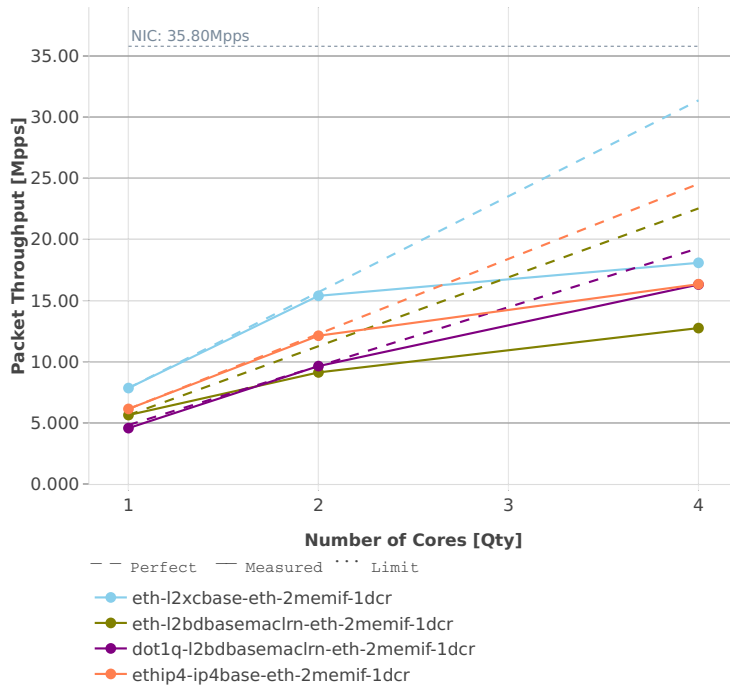
Speedup Multi-core: memif-2n-skx-xxv710-64b-base_and_features-ndr
