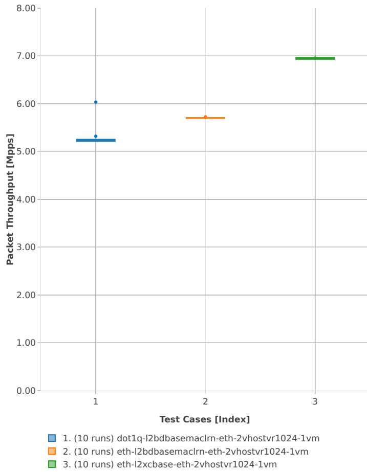
Throughput: vhost-l2sw-2n-skx-xxv710-64b-2t1c-base_and_features-pdr
