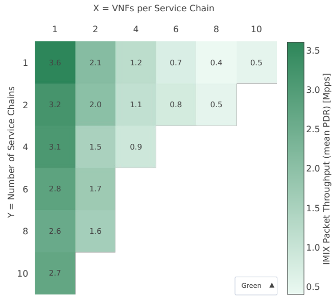
Throughput: eth-l2bd-{2XY}vhost-{Y}chain-{XY}vm-l3fwdip4-pdr
