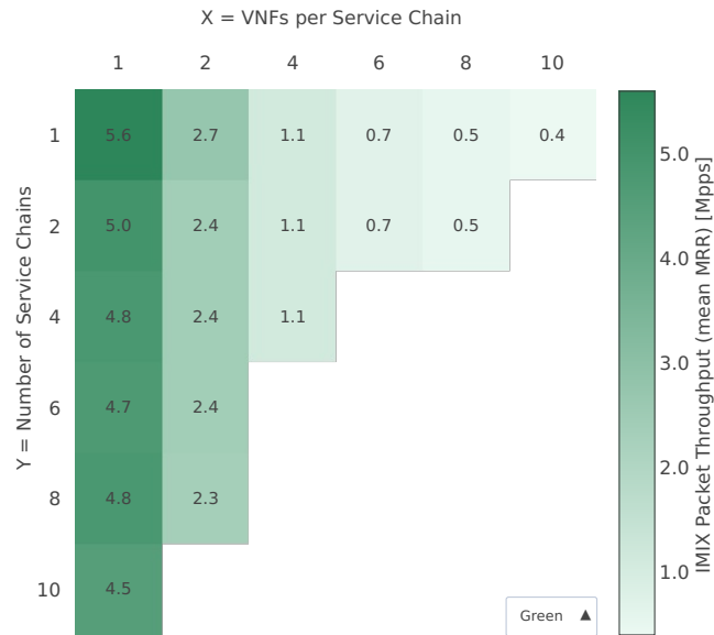
Throughput: eth-l2bd-{2XY}vhost-{Y}chain-{XY}vm-l3fdip4-mrr
