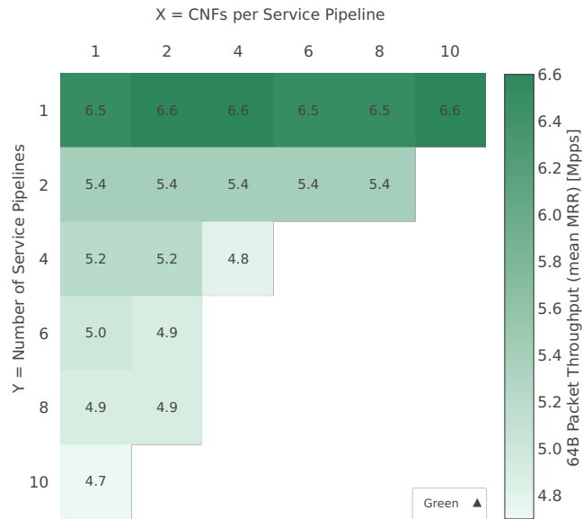
Throughput: eth-l2bd-{2Y}memif-{Y}pipe-{XY}drc-vppip4-mrr
