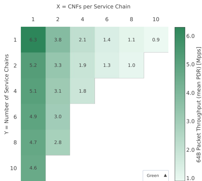
Throughput: eth-l2bd-{2XY}memif-{Y}chain-{XY}drc-vppip4-pdr
