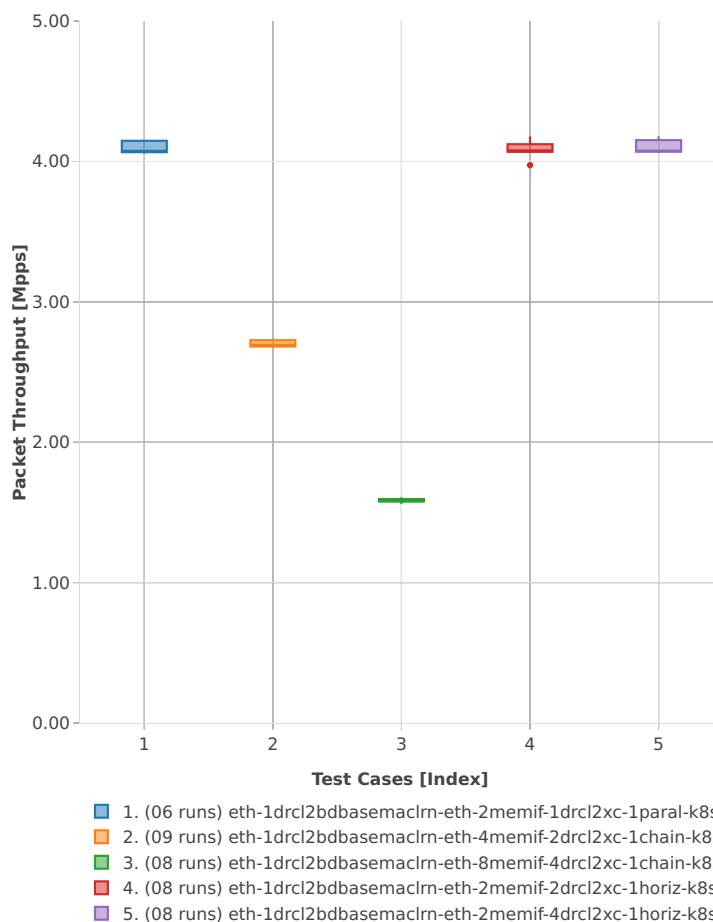
Throughput: k8s-memif-3n-hsw-x710-64b-1t1c-base_and_scale-l2bd-ndr
