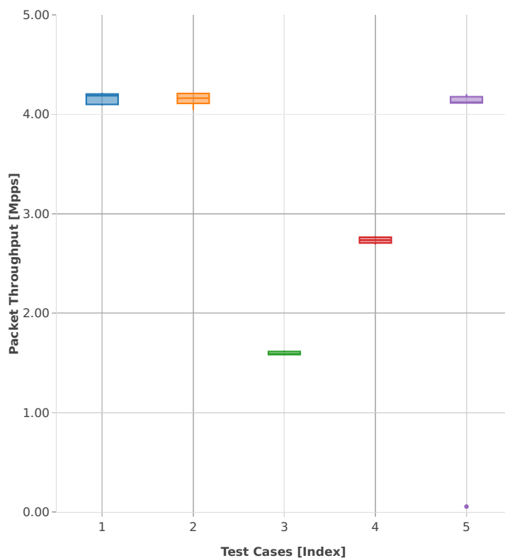
Throughput: k8s-memif-3n-hsw-x520-64b-1t1c-base_and_scale-l2bd-ndr
