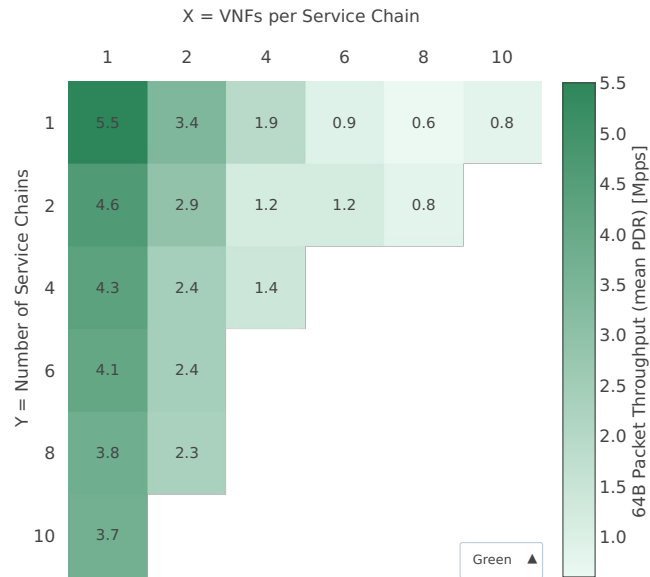
Throughput: eth-l2bd-{2XY}vhost-{Y}chain-{XY}vm-l3fwdip4-pdr
