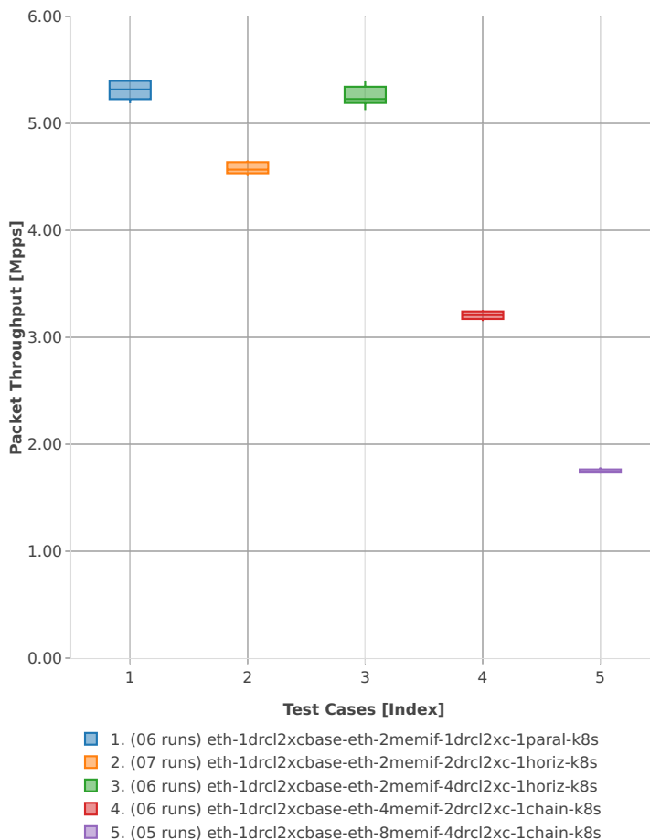
Throughput: k8s-memif-3n-hsw-x710-64b-1t1c-base_and_scale-l2xc-ndr
