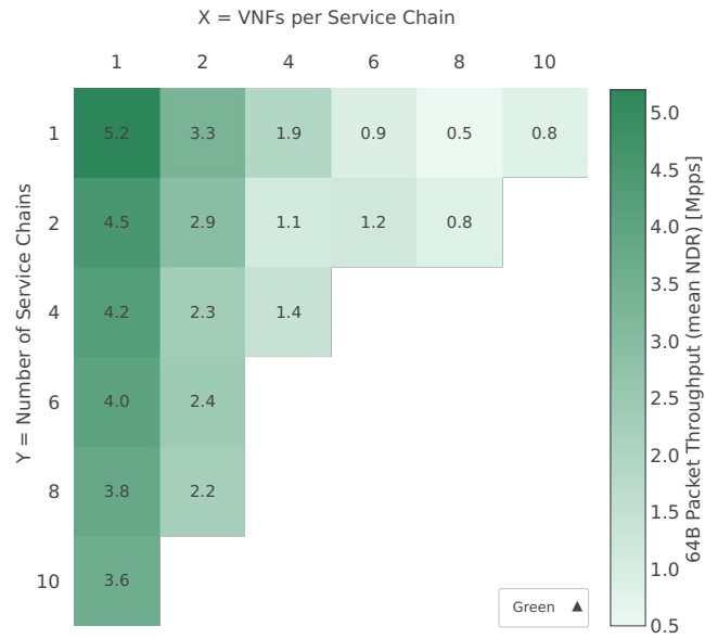
Throughput: eth-l2bd-{2XY}vhost-{Y}chain-{XY}vm-l3fwdip4-ndr
