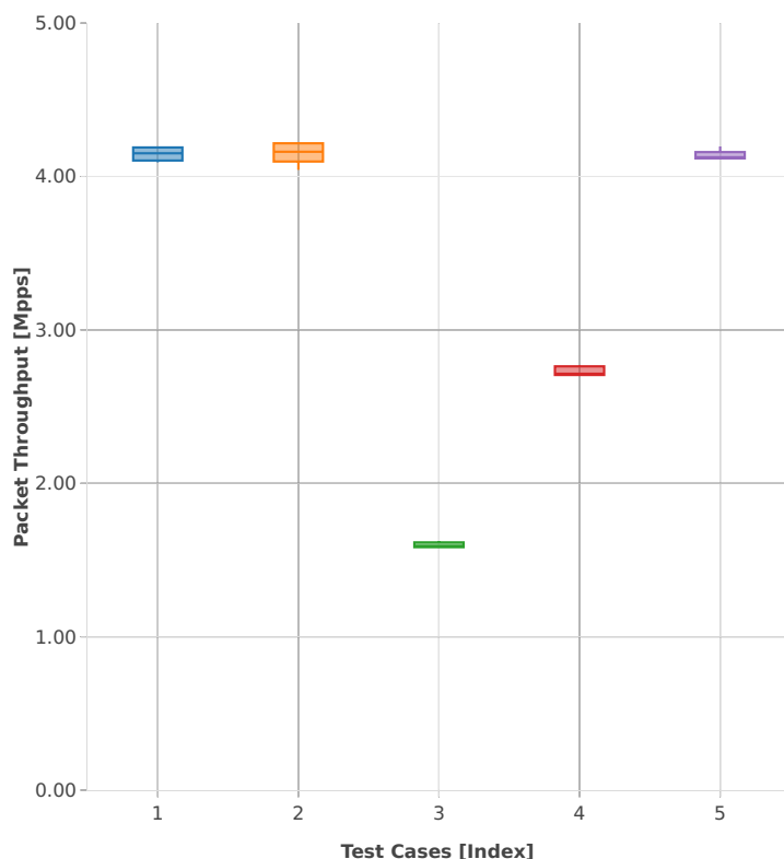
Throughput: k8s-memif-3n-hsw-x520-64b-1t1c-base_and_scale-l2bd-ndr
