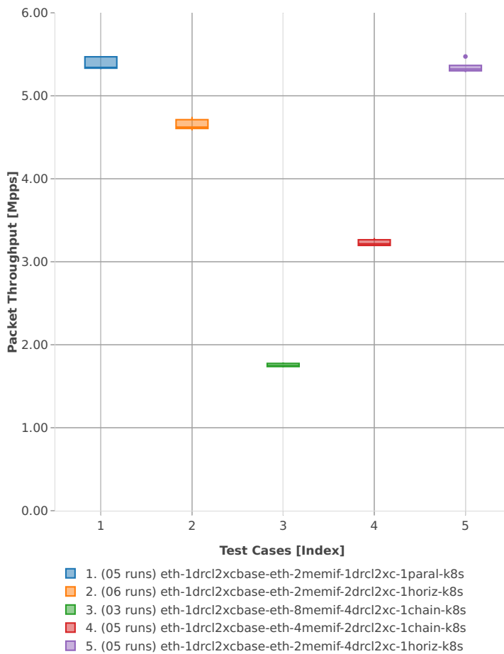
Throughput: k8s-memif-3n-hsw-x520-64b-1t1c-base_and_scale-l2xc-ndr
