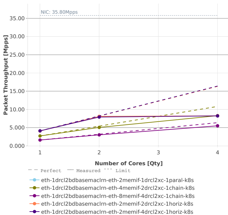
Speedup Multi-core: k8s-memif-3n-hsw-x710-64b-base_and_scale-l2bd-ndr
