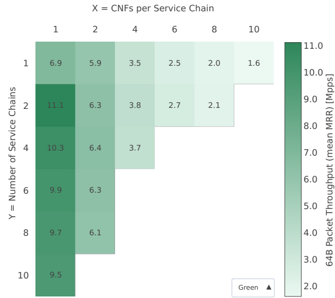
Throughput: eth-l2bd-{2XY}memif-{Y}chain-{XY}drc-vppip4-mrr
