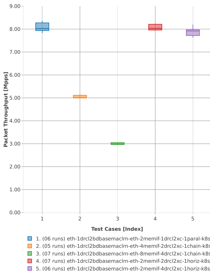
Throughput: k8s-memif-3n-hsw-x710-64b-2t2c-base_and_scale-l2bd-ndr
