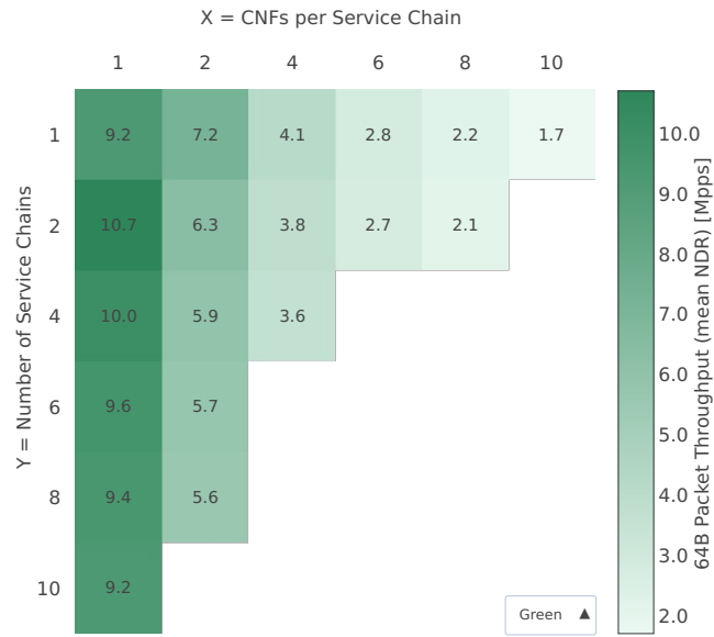
Throughput: eth-l2bd-{2XY}memif-{Y}chain-{XY}drc-vppip4-ndr
