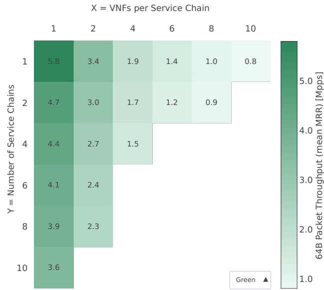
Throughput: eth-l2bd-{2XY}vhost-{Y}chain-{XY}vm-l3fdip4-mrr
