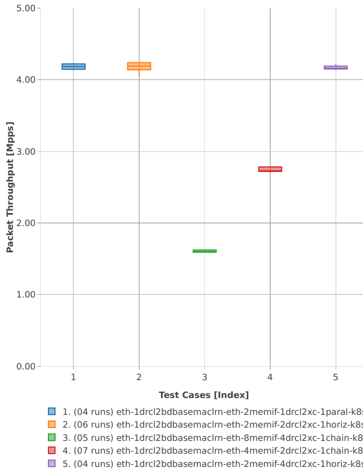
Throughput: k8s-memif-3n-hsw-x520-64b-1t1c-base_and_scale-l2bd-pdr
