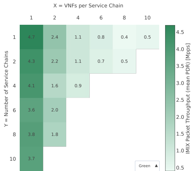
Throughput: eth-l2bd-{2XY}vhost-{Y}chain-{XY}vm-l3fdip4-pdr
