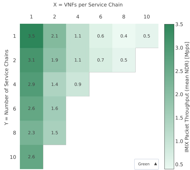
Throughput: eth-l2bd-{2XY}vhost-{Y}chain-{XY}vm-l3fdip4-ndr
