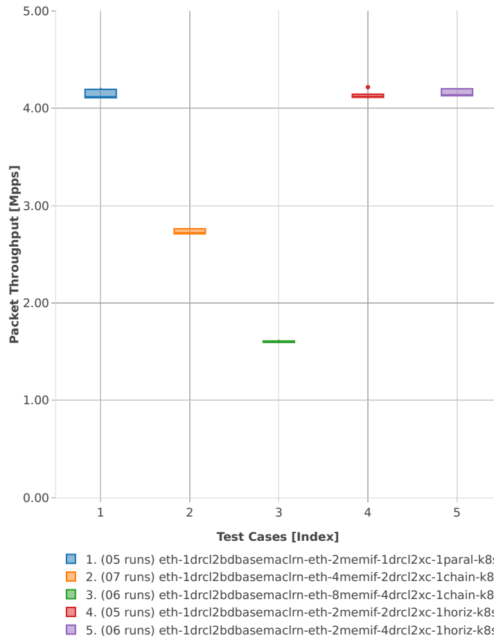
Throughput: k8s-memif-3n-hsw-x710-64b-1t1c-base_and_scale-l2bd-pdr
