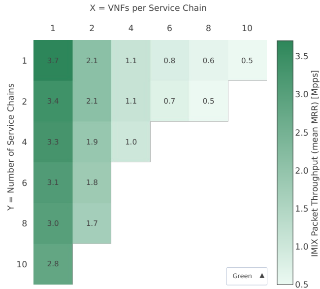
Throughput: eth-l2bd-{2XY}vhost-{Y}chain-{XY}vm-l3fdip4-mrr
