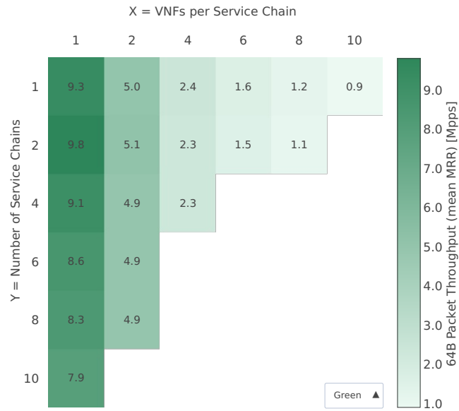
Throughput: eth-l2bd-{2XY}vhost-{Y}chain-{XY}vm-l3fdip4-mrr
