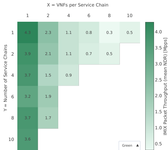
Throughput: eth-l2bd-{2XY}vhost-{Y}chain-{XY}vm-l3fdip4-ndr
