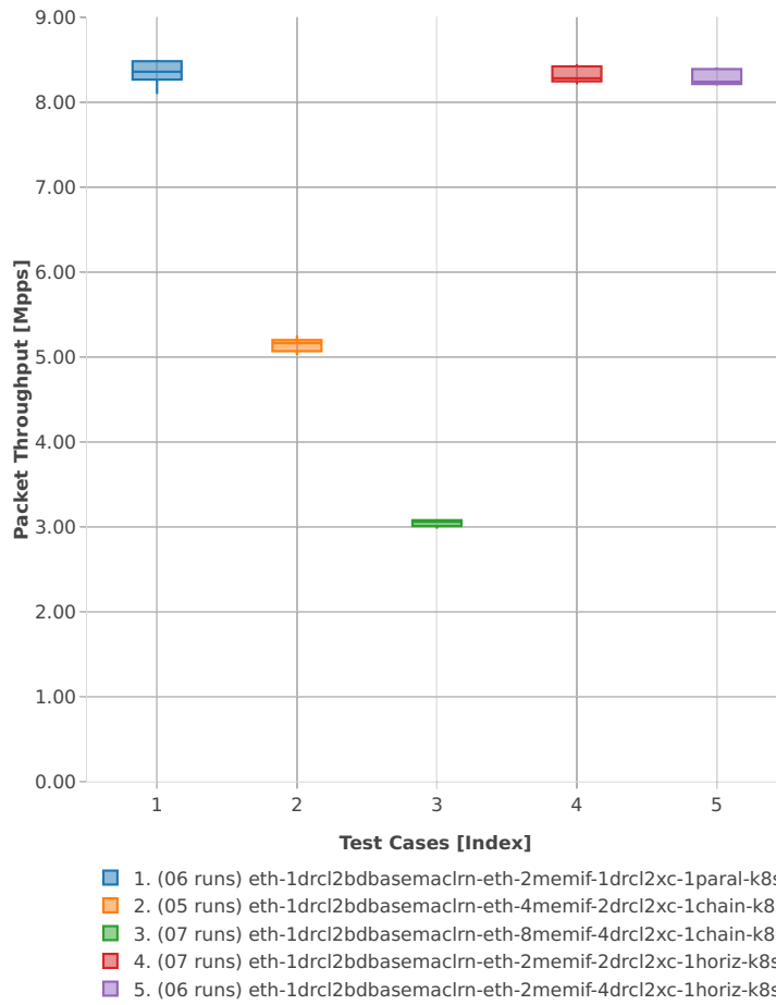
Throughput: k8s-memif-3n-hsw-x710-64b-2t2c-base_and_scale-l2bd-pdr
