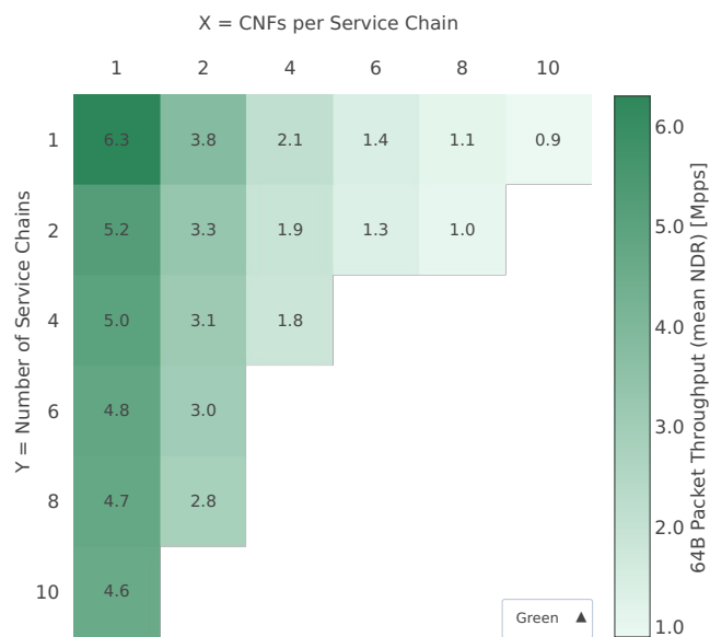
Throughput: eth-l2bd-{2XY}memif-{Y}chain-{XY}drc-vppip4-ndr
