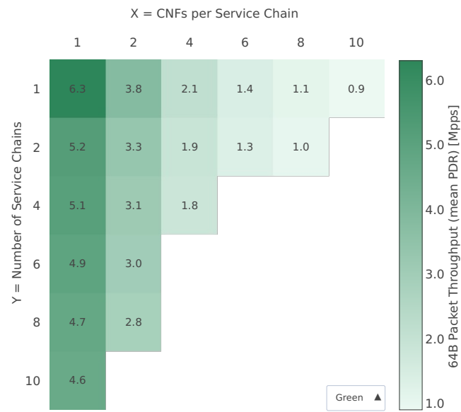
Throughput: eth-l2bd-{2XY}memif-{Y}chain-{XY}drc-vppip4-pdr
