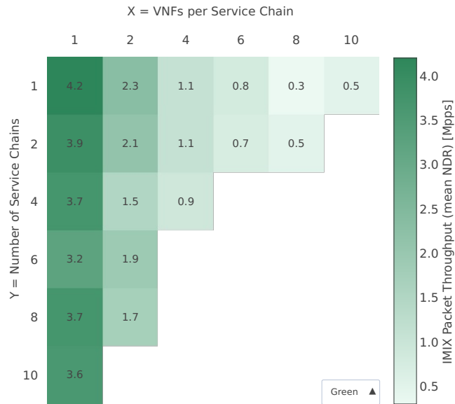
Throughput: eth-l2bd-{2XY}vhost-{Y}chain-{XY}vm-l3fdip4-ndr
