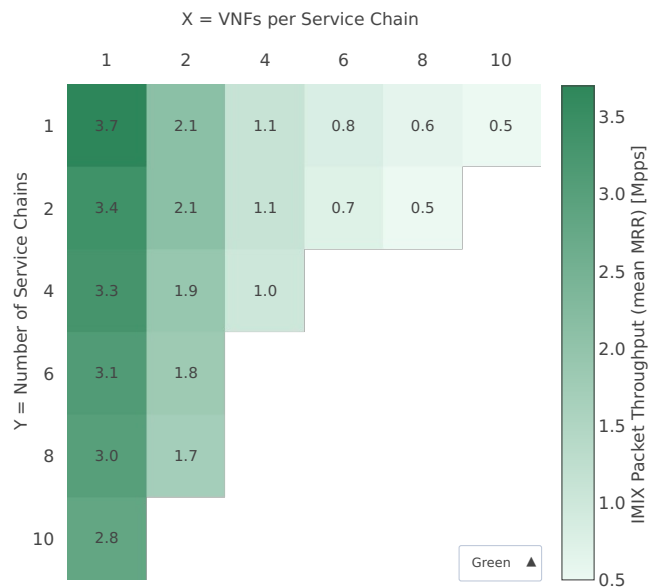
Throughput: eth-l2bd-{2XY}vhost-{Y}chain-{XY}vm-l3fdip4-mrr
