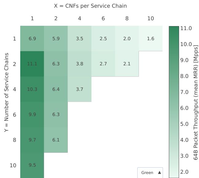
Throughput: eth-l2bd-{2XY}memif-{Y}chain-{XY}drc-vppip4-mrr
