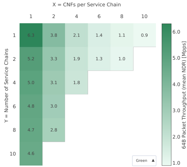
Throughput: eth-l2bd-{2XY}memif-{Y}chain-{XY}drc-vppip4-ndr
