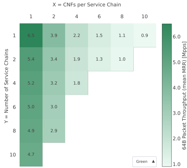
Throughput: eth-l2bd-{2XY}memif-{Y}chain-{XY}drc-vppip4-mrr
