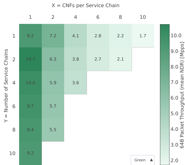
Throughput: eth-l2bd-{2XY}memif-{Y}chain-{XY}drc-vppip4-ndr
