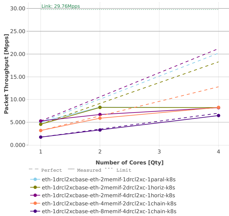
Speedup Multi-core: k8s-memif-3n-hsw-x710-64b-base_and_scale-l2xc-pdr
