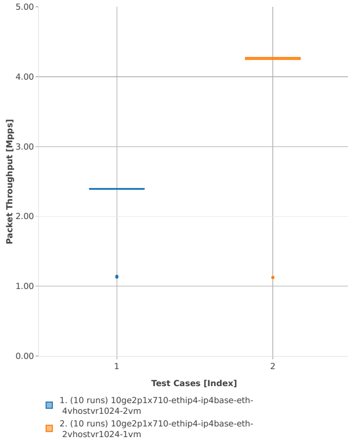
Packet Throughput: vhost-ip4-3n-hsw-x710-64b-1t1c-base_and_scale-ndr
