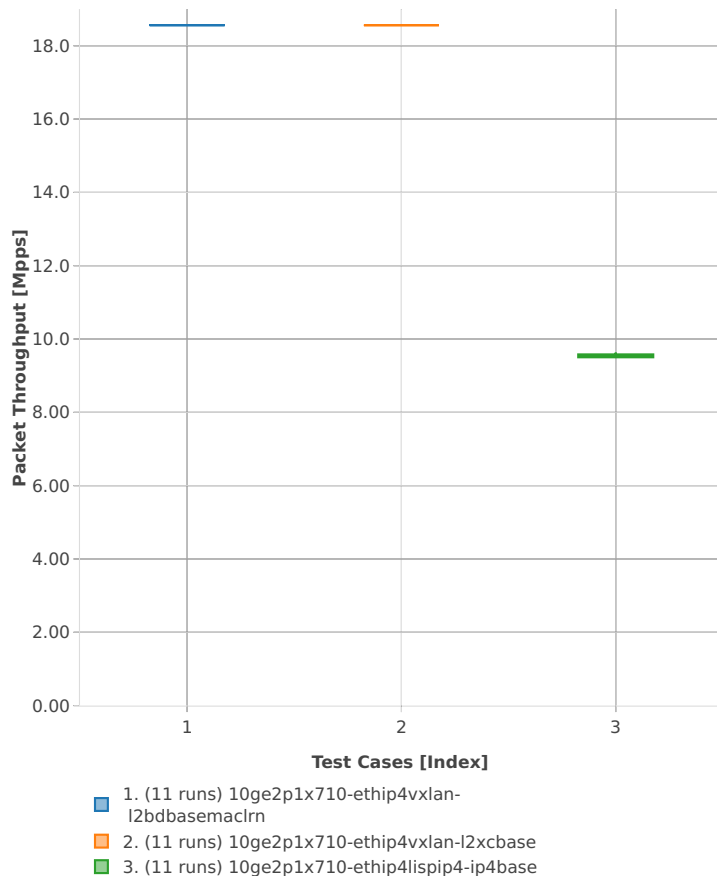
Packet Throughput: ip4tun-3n-skx-x710-64b-4t2c-base_and_features-ndr
