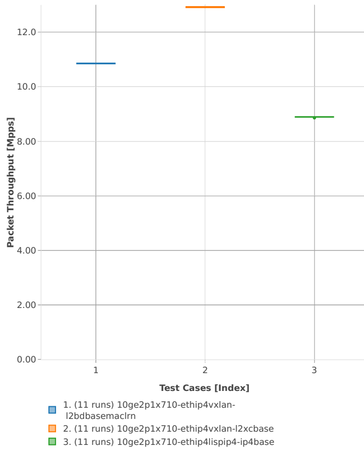
Packet Throughput: ip4tun-3n-skx-x710-64b-2t1c-base_and_features-pdr
