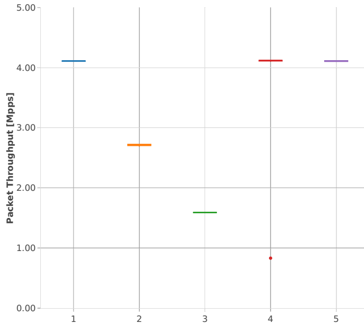
Packet Throughput: k8s-memif-3n-hsw-x710-64b-1t1c-base_and_scale-l2bd-p
