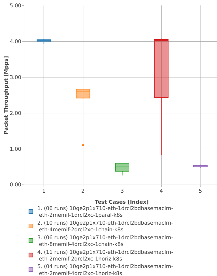
Packet Throughput: k8s-memif-3n-hsw-x710-64b-1t1c-base_and_scale-l2bd-n
