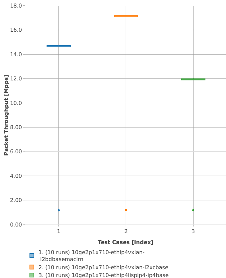
Packet Throughput: ip4tun-3n-hsw-x710-64b-2t2c-base_and_features-ndr
