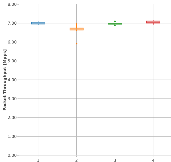
Packet Throughput: vhost-l2sw-3n-skx-x710-64b-4t2c-base_and_scale-ndr
