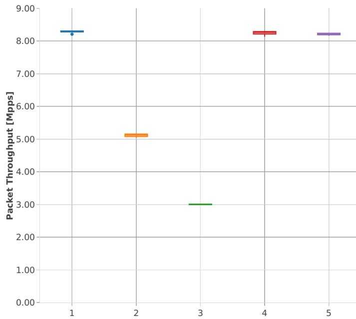
Packet Throughput: k8s-memif-3n-hsw-x710-64b-2t2c-base_and_scale-l2bd-p
