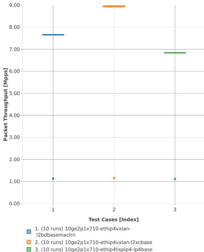
Packet Throughput: ip4tun-3n-hsw-x710-64b-1t1c-base_and_features-ndr
