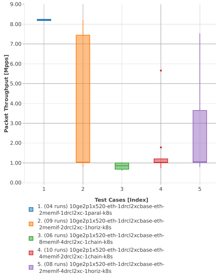
Packet Throughput: k8s-memif-3n-hsw-x520-64b-2t2c-base_and_scale-l2xc-n
