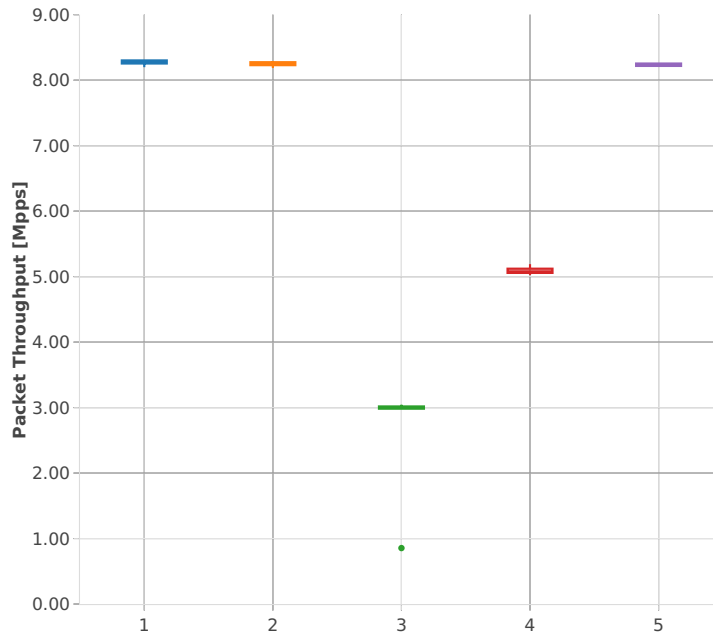
Packet Throughput: k8s-memif-3n-hsw-x520-64b-2t2c-base_and_scale-l2bd-p
