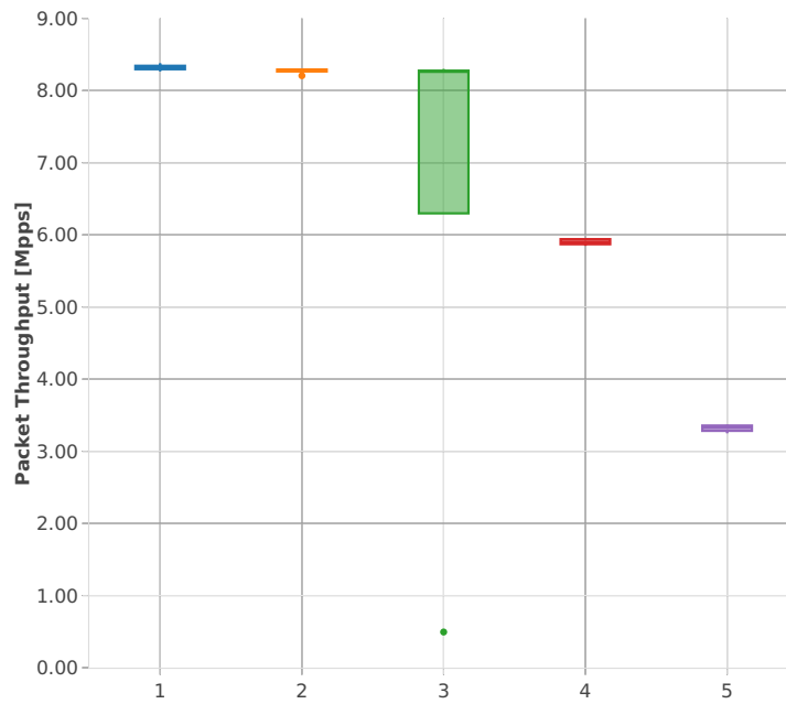
Packet Throughput: k8s-memif-3n-hsw-x710-64b-2t2c-base_and_scale-l2xc-p
