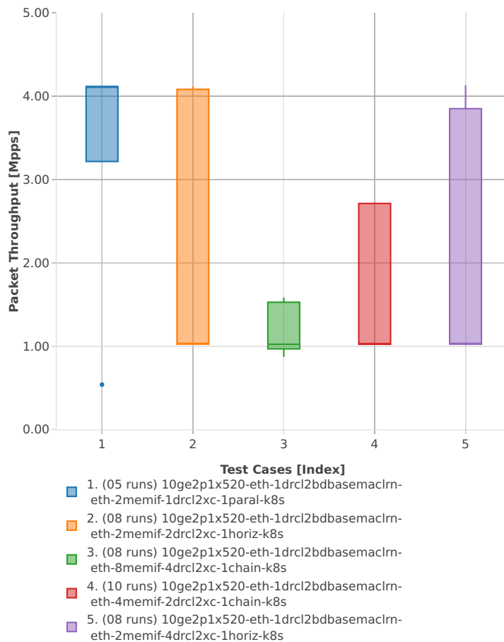
Packet Throughput: k8s-memif-3n-hsw-x520-64b-1t1c-base_and_scale-l2bd-n
