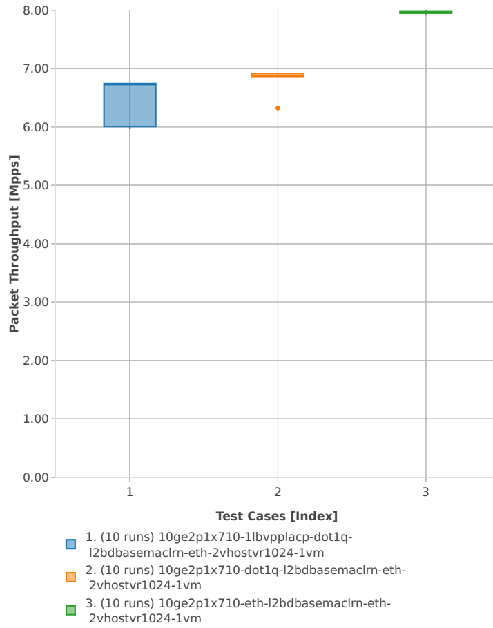
Packet Throughput: vhost-l2sw-3n-hsw-x710-64b-2t2c-base_and_scale-pdr
