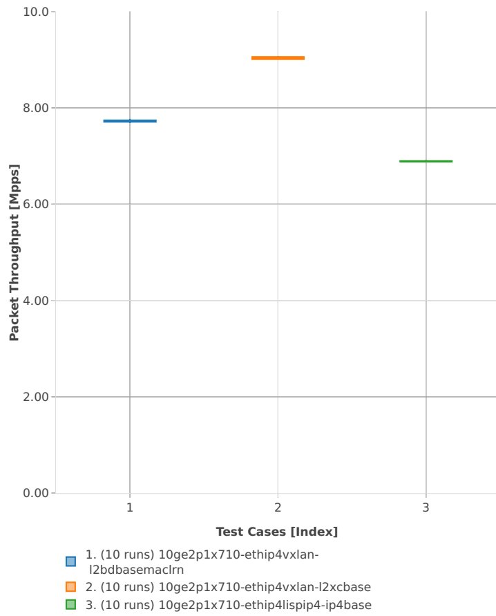
Packet Throughput: ip4tun-3n-hsw-x710-64b-1t1c-base_and_features-pdr
