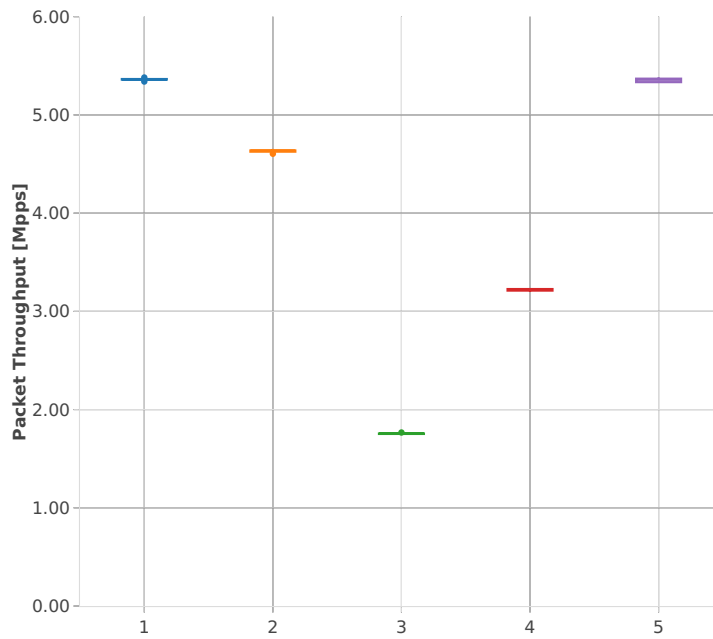
Packet Throughput: k8s-memif-3n-hsw-x520-64b-1t1c-base_and_scale-l2xc-p
