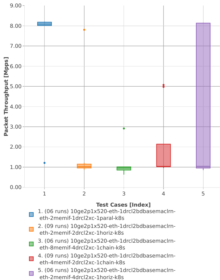
Packet Throughput: k8s-memif-3n-hsw-x520-64b-2t2c-base_and_scale-l2bd-n
