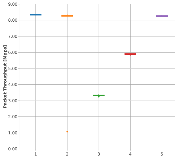
Packet Throughput: k8s-memif-3n-hsw-x520-64b-2t2c-base_and_scale-l2xc-p
