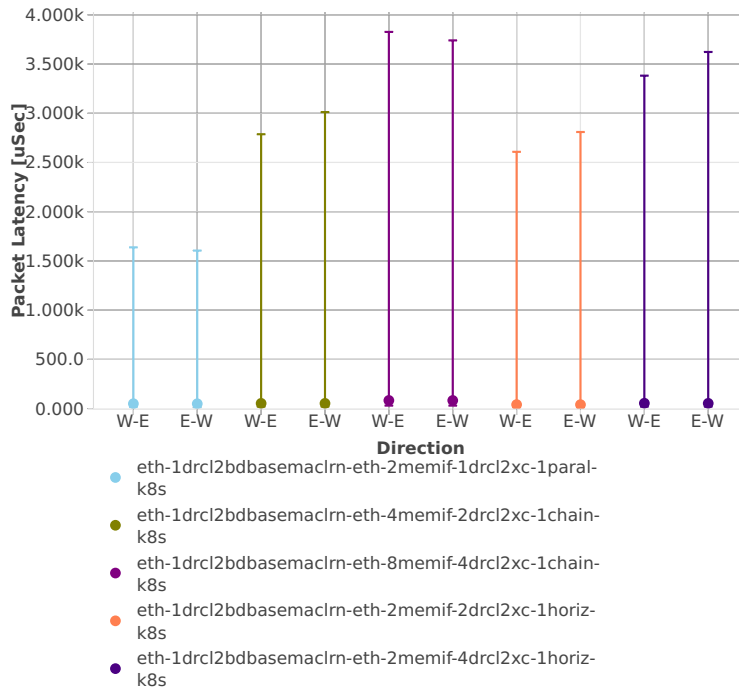
Packet Latency: k8s-memif-3n-hsw-x710-64b-2t2c-base_and_scale-l2bd-ndr
