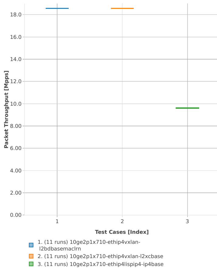
Packet Throughput: ip4tun-3n-skx-x710-64b-4t2c-base_and_features-pdr
