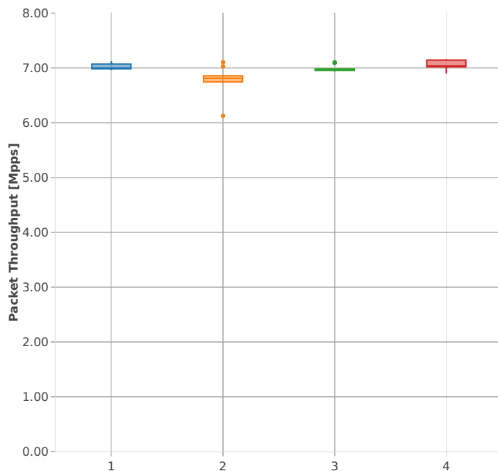
Packet Throughput: vhost-l2sw-3n-skx-x710-64b-4t2c-base_and_scale-pdr
