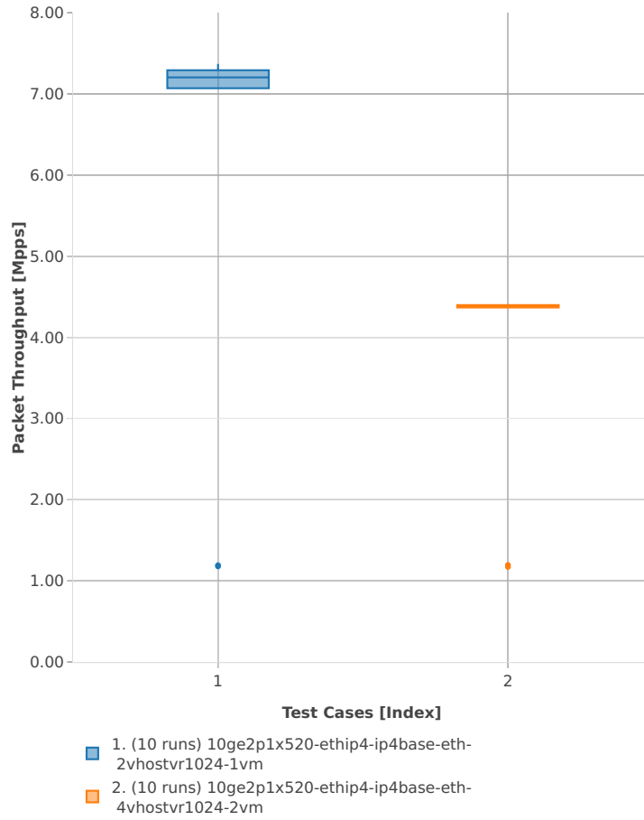
Packet Throughput: vhost-ip4-3n-hsw-x520-64b-2t2c-base_and_scale-ndr
