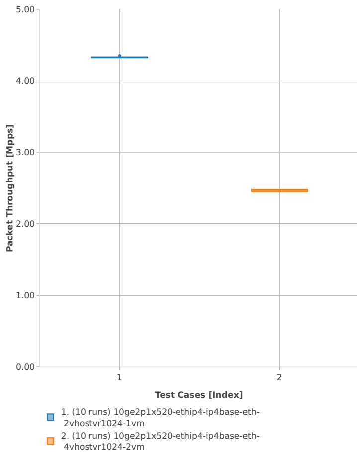
Packet Throughput: vhost-ip4-3n-hsw-x520-64b-1t1c-base_and_scale-pdr
