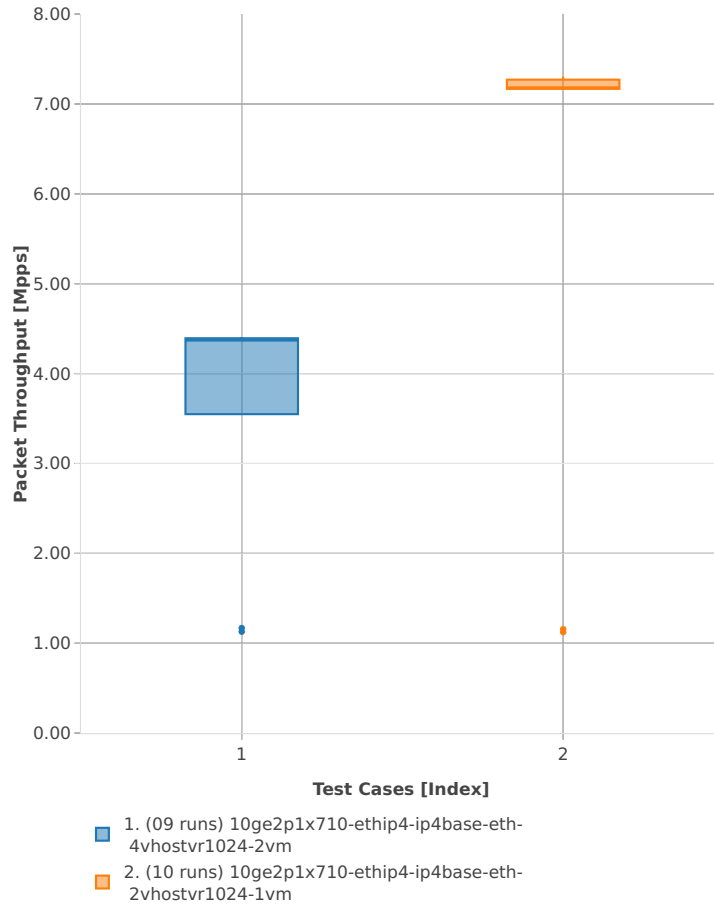
Packet Throughput: vhost-ip4-3n-hsw-x710-64b-2t2c-base_and_scale-ndr
