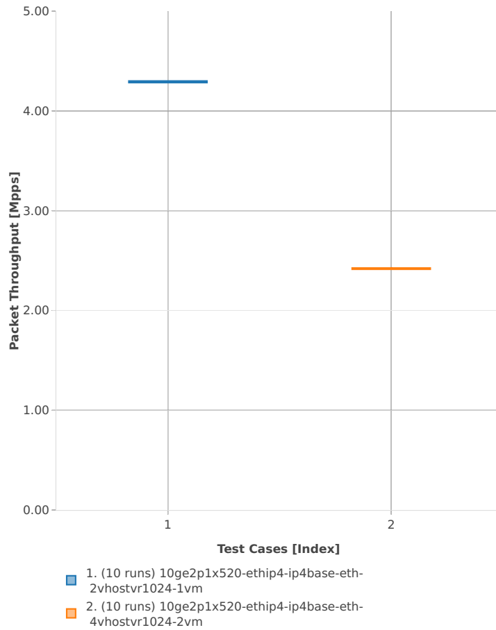
Packet Throughput: vhost-ip4-3n-hsw-x520-64b-1t1c-base_and_scale-ndr
