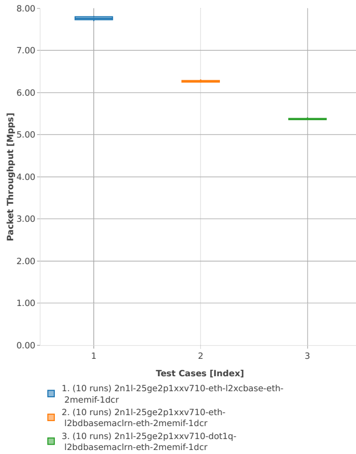
Packet Throughput: memif-2n-skx-xxv710-64b-2t1c-base_and_scale-pdr
